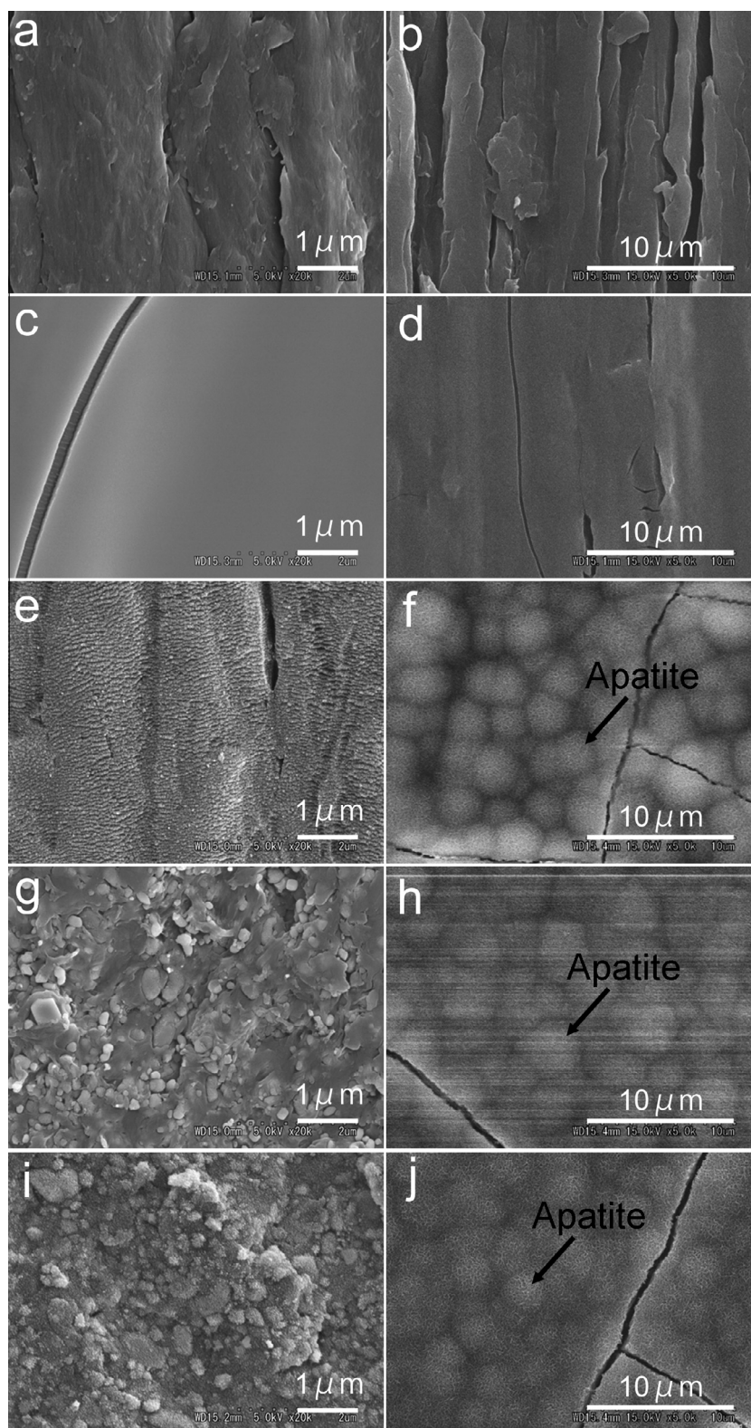
Fig. 2. SEM images of surface-coated PEEK samples. (a) Uncoated PEEK, showing polishing traces on the surface, (b) uncoated PEEK, after soaking in SBF. (c) OS, showing the smooth sol-gel coating layer (d) OS, after soaking in SBF. (e) OSH, showing fine precipitation on the surface, (f) OSH, after soaking in SBF (g) BH, showing a nano-scale rough surface, (h) BH, after soaking in SBF. (i) BSH, showing fine precipitation on a nano-scale rough surface (j) BSH after soaking in SBF. Dome-shaped apatite formation was observed in the OSH, BH, and BSH groups (f, h, j).
