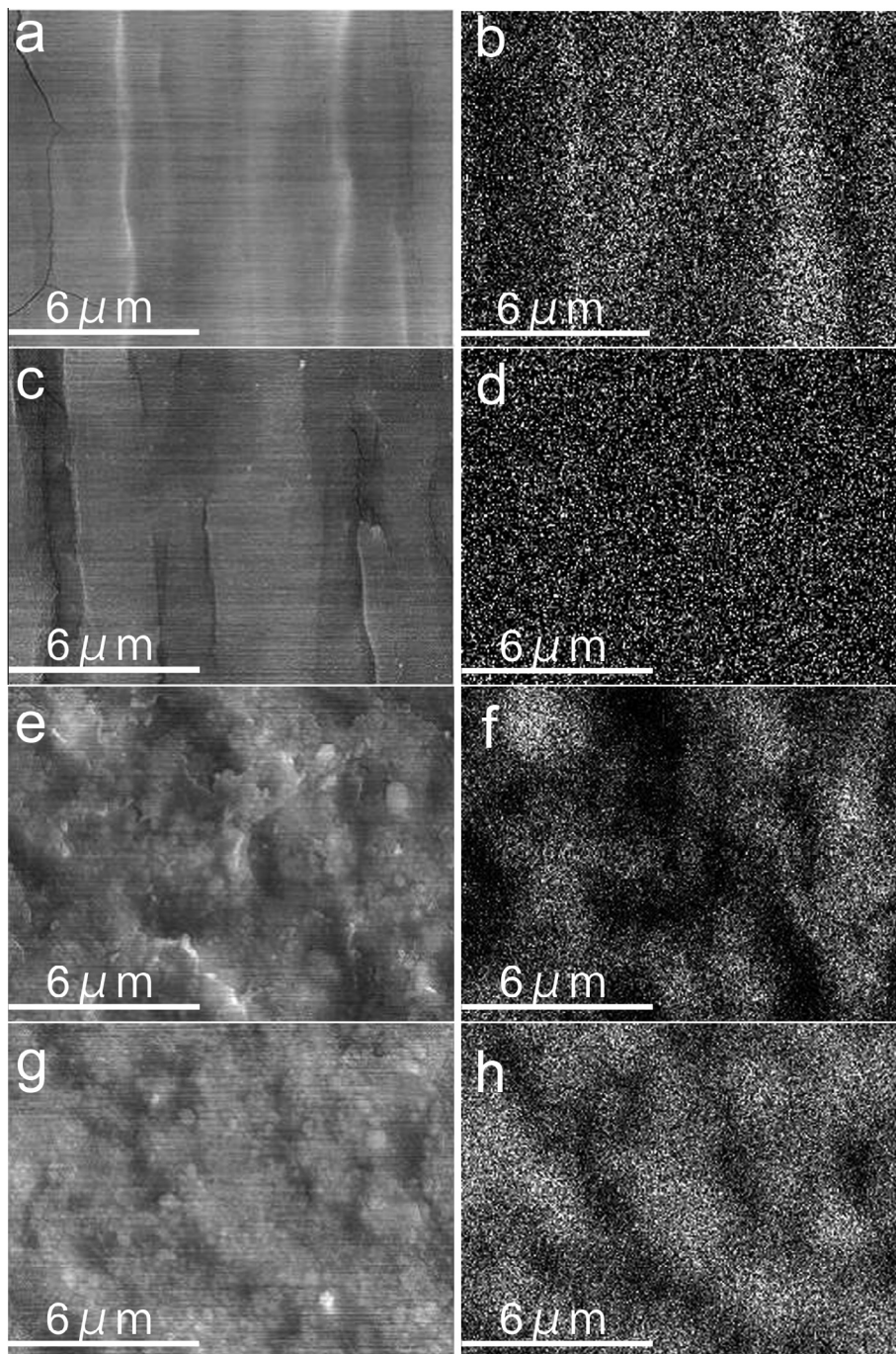
Fig. 3. The titanium distributions of coated surfaces. (a, c, e, g) SEM images of OS, OSH, BH, BSH, respectively. (b, d, f, h) Titanium distribution by EDX for (a, c, e, g), respectively. A non-uniform titanium distribution exists in OS and BH group (b, f). The non-uniformity was improved by acid post-treatment (d) and a sol-gel coating with acid post-treatment (h).
