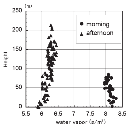
Fig. 3. The vertical distribution of the absolute humidity by the observation using a kite.
