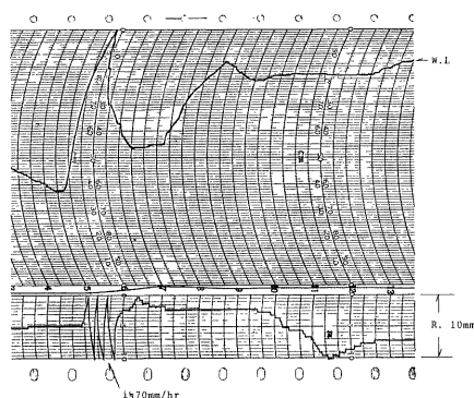
Fig. 8 An actual example of simultaneous records of water-stage and rainfall, Type D. The water gauge has been installed at a point of the drainage channel, the Ogura basin.
