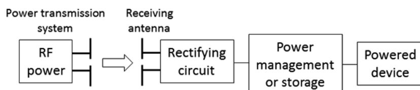
Figure 1. Block diagram of a MPT system.
