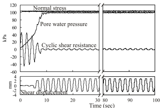
Fig. 2 Results of undrained cyclic shear stress-controlled ring-shear test on mixture of S7 with 7% bentonite (B7)
