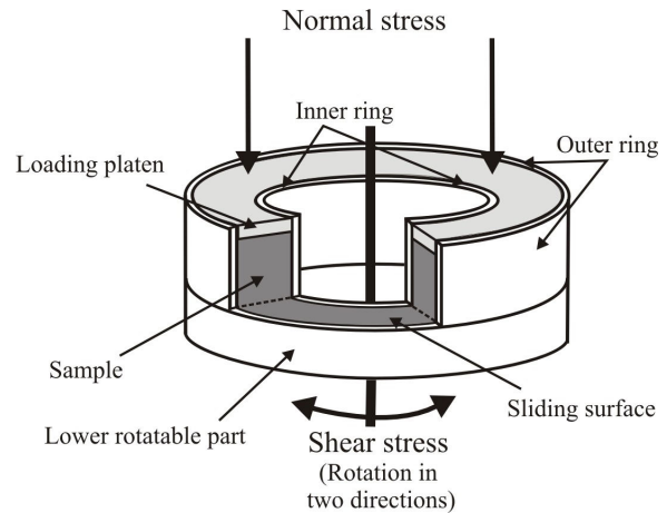
Fig. 1 The undrained cyclic ring-shear box.
