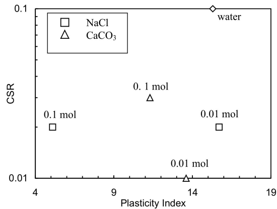
Fig. 4 Results of the second series of ring-shear tests plotted as plasticity index against CSR
