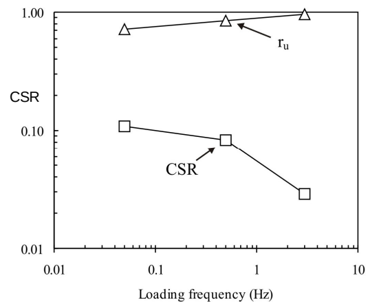
Fig. 5 Results of the third series of ring-shear tests plotted as loading frequency against CSR and r_u
