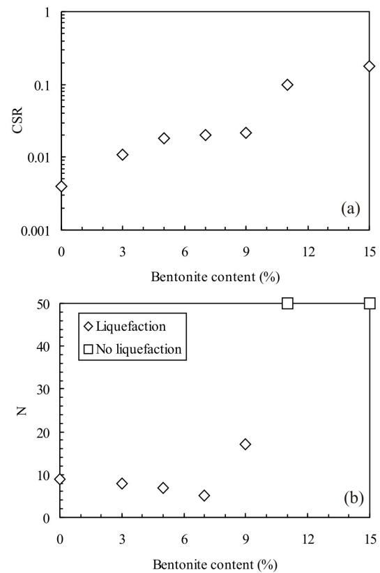
Fig. 3 Results of the first series of ring-shear tests plotted as bentonite content against CSR (a), and bentonite content against N (b)
