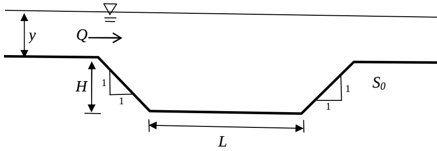
Fig.2.12 Sketch of the mining pit.
