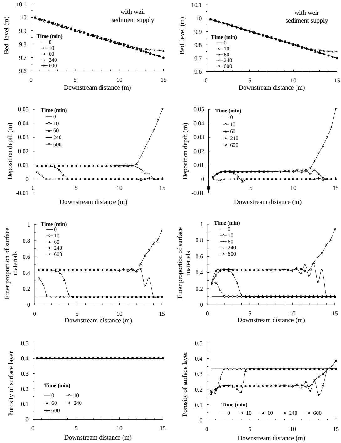
Fig.5.26 Simulation result on bed and porosity variation of binary mixtures, Case B-4 (with weir and sediment supply); (a) porosity is assumed to be constant, (b) porosity is calculated by Eqs.(5.10) and (5.11).
