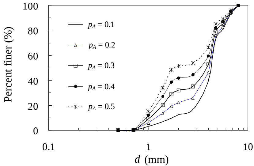
Fig.4.19 Average observed distribution of five bimodal distributions with different proportion of material A, p_A .
