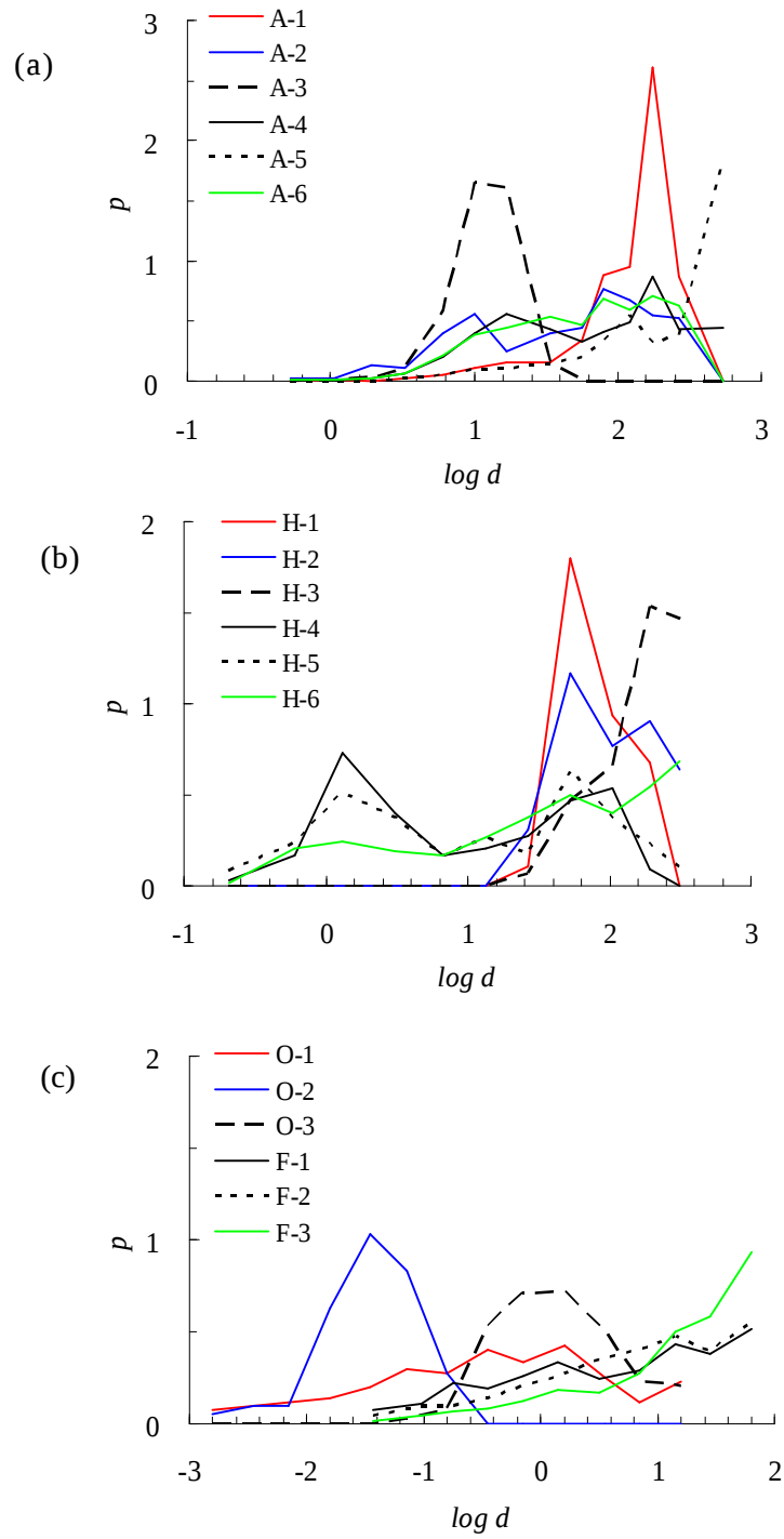
Fig.3.12 Probability density distributions of natural sediment mixtures sampled in (a) Ai River, (b) Hino River and (c) Ohtaki River and a Fukadani bare slope.
