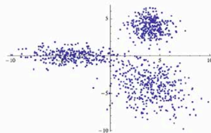
(b) Data sampled from this distribution.
