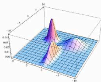
(a) A probability distribution on \mathbb{R}^2 .
