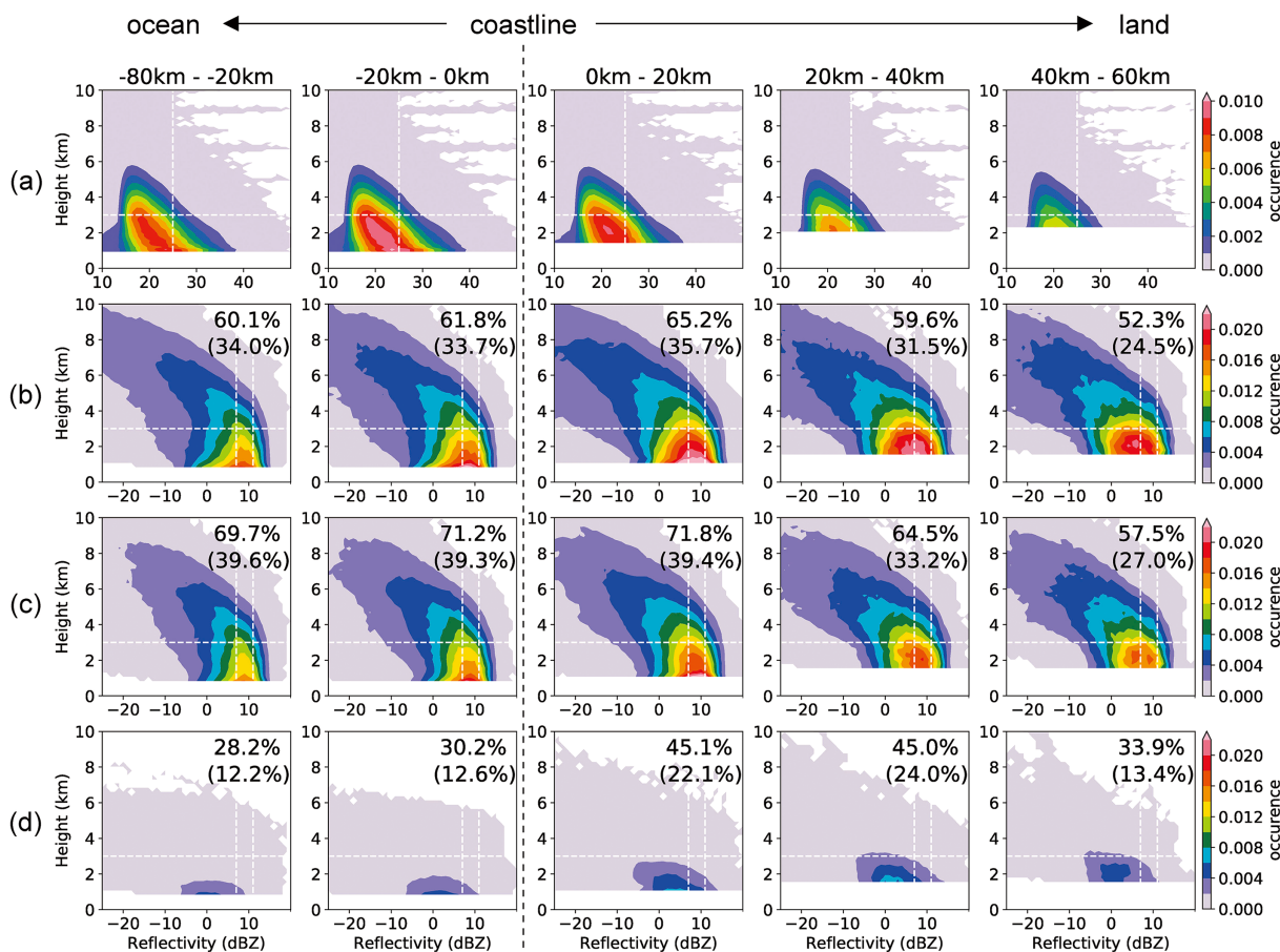
Fig. 7. CFADs of (a) the 5-year-mean KuPR reflectivity and the 4-year-mean CPR reflectivity of (b) all, (c) nimbostratus, and (d) shallow cumuliform cloud types when precipitation is detected for different distances from the coastline. Two-dimensional histograms of the reflectivity profile with intervals of 1 dB and a vertical resolution of (a) 125 m and (b–d) 240 m. Each CFAD is normalized by the number of observations in the respective area. White dashed vertical lines at reflectivity of 7 dBZ (11 dBZ) in (b–d) indicate the threshold at which KuPR detects the echo over the ocean (over the coastal mountains). For all CFADs of the CPR, the ratio of the number of profiles with echoes stronger than the 7-dBZ and 11-dBZ thresholds to the total number of observed profiles is calculated and shown in the upper right of each CFAD. (The ratio when the 11-dBZ threshold is applied is shown in parentheses.) White dashed horizontal lines at a height of 3 km and vertical lines at 25 dBZ in (a) are drawn for reference.
