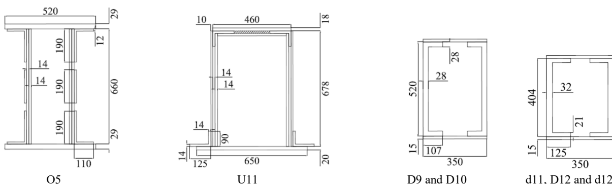
Fig.15 Estimated cross sections of three span truss with suspension truss structure to support full live load (Dimensions in mm).
