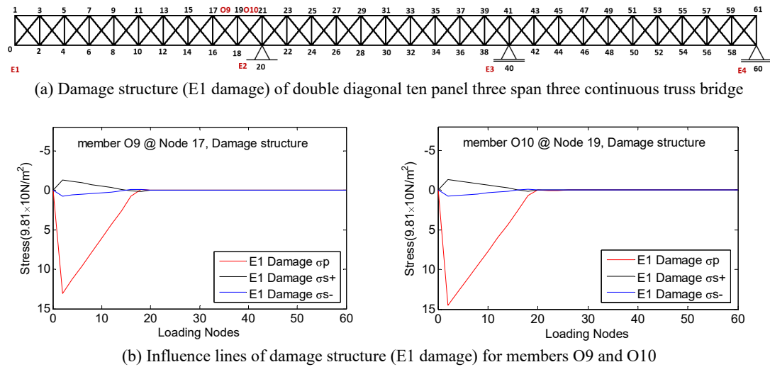
Fig.8 Influence lines of damage structure (E1 damage) for members O9 and O10 in ten panel three span continuous truss bridge.
