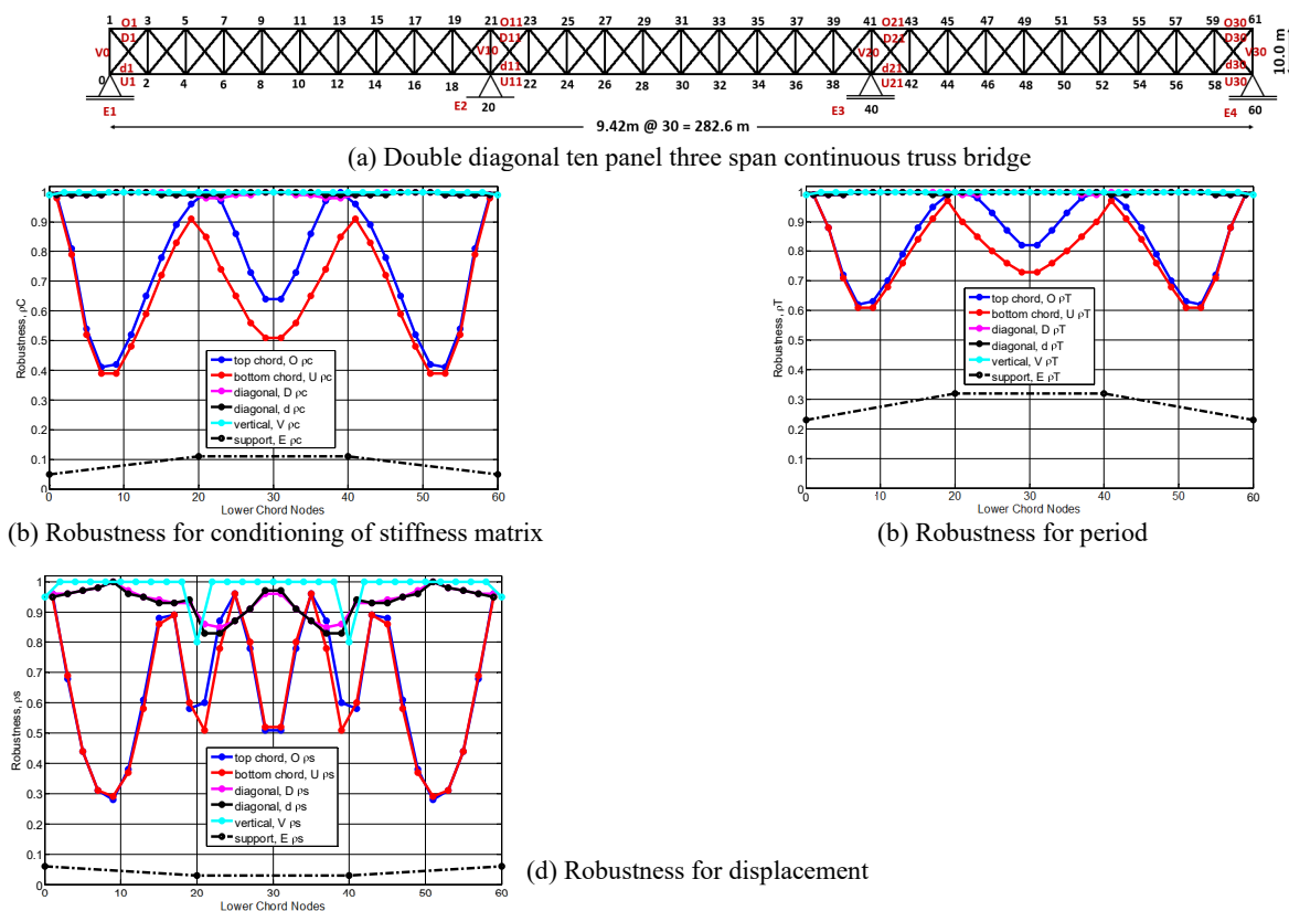
Fig.4 Robustness indices of ten panel three span continuous truss bridge for damage of one member and external support.
