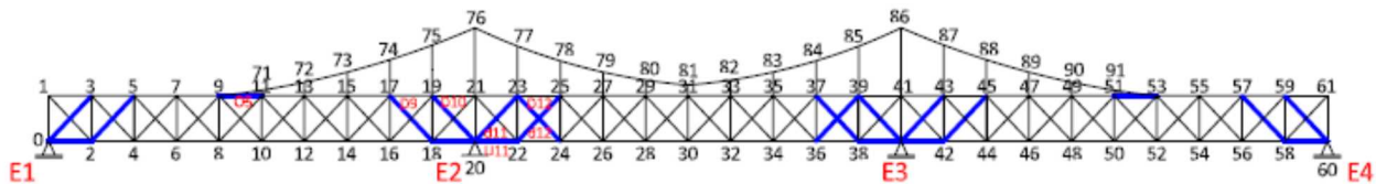
Fig.17 Ten panel three span continuous truss with suspension truss structure including segments and node numbers.
