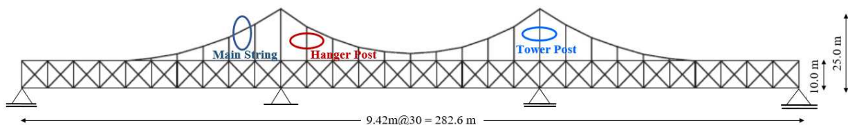
(b) Longitudinal profile for proposed bridge
