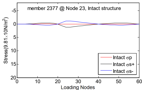
(c) Influence lines for hanger post
