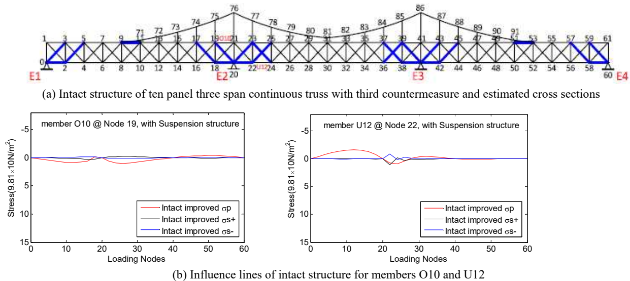
Fig.20 Influence lines of intact structure for members O10 and U12 in ten panel three span continuous truss bridge with third countermeasure and estimated cross sections.
