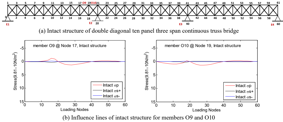
Fig.7 Influence lines of intact structure for members O9 and O10 in ten panel three span continuous truss bridge.
