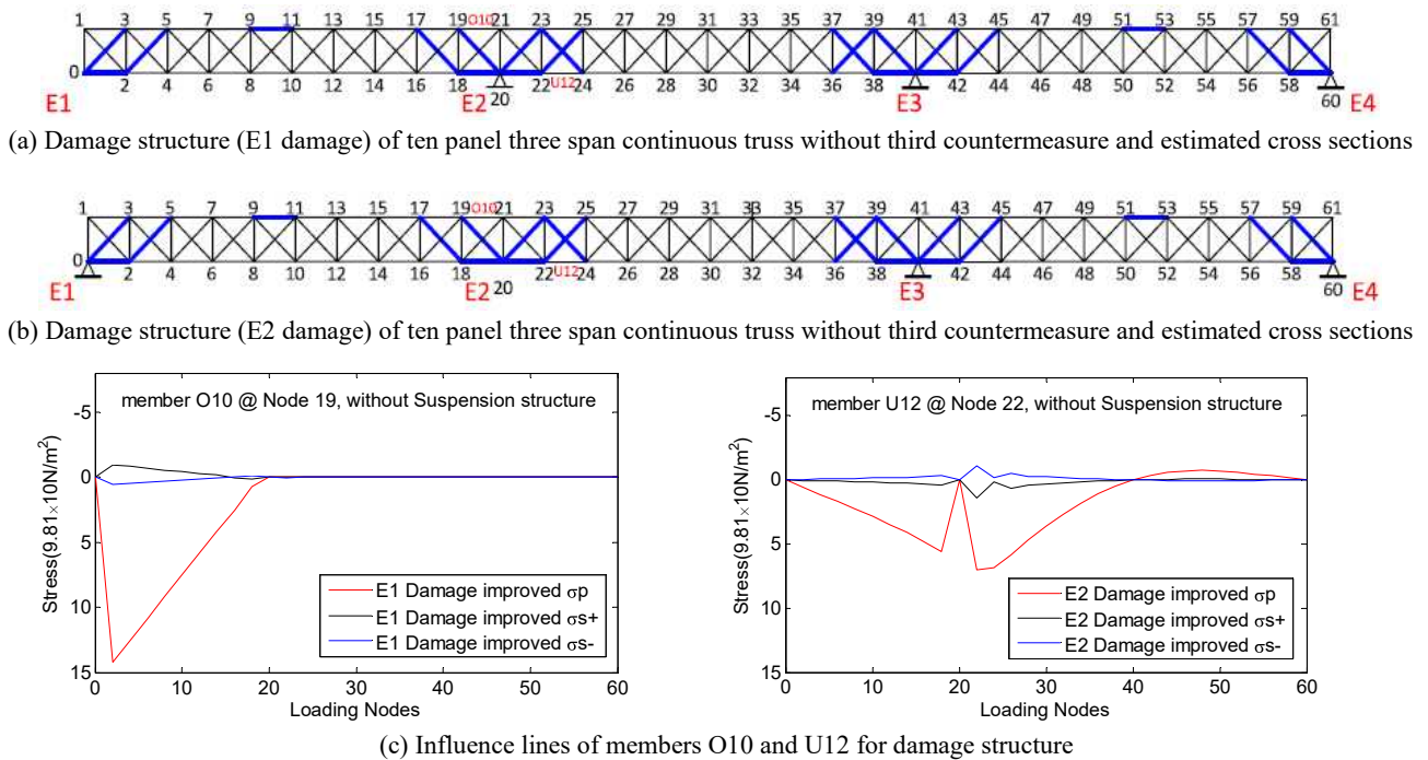
Fig.23 Influence lines of damage structures for members O10 (E1 damage) and U12 (E2 damage) in ten panel three span continuous truss bridge without third countermeasure and estimated cross sections.
