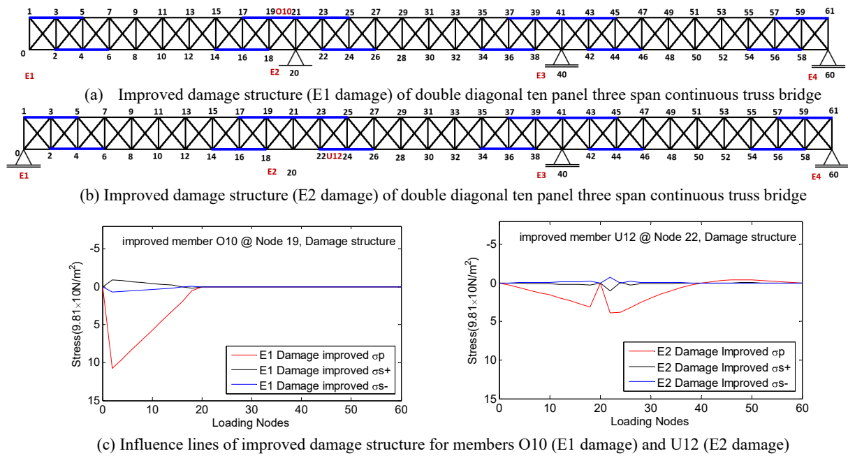
Fig.10 Influence lines of improved damage structure for members O10 and U12 in ten panel three span continuous truss bridge.
