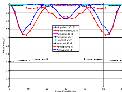
(b) Robustness for period
