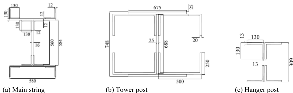
Fig.14 Proposed estimated cross sections for suspension truss structure (Dimensions in mm).
