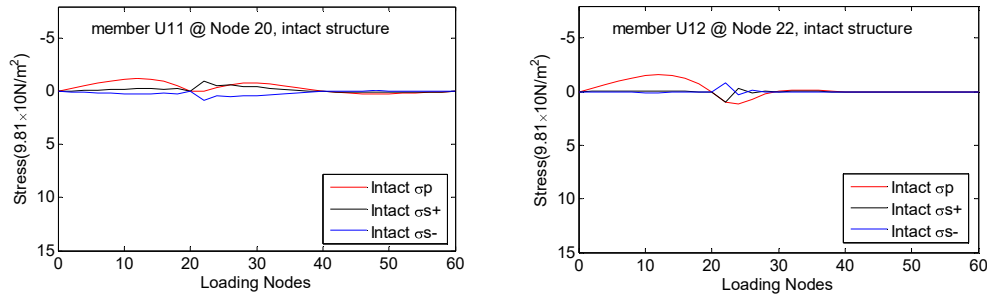
(b) Influence lines of intact structure for members U11 and U12
