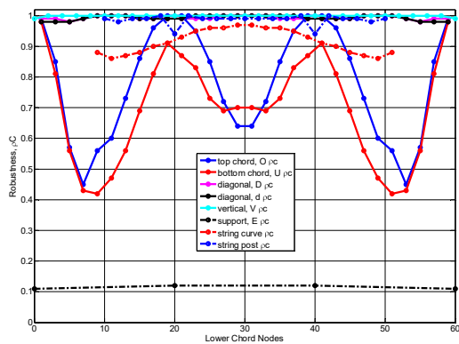
(a) Robustness for conditioning of stiffness matrix
