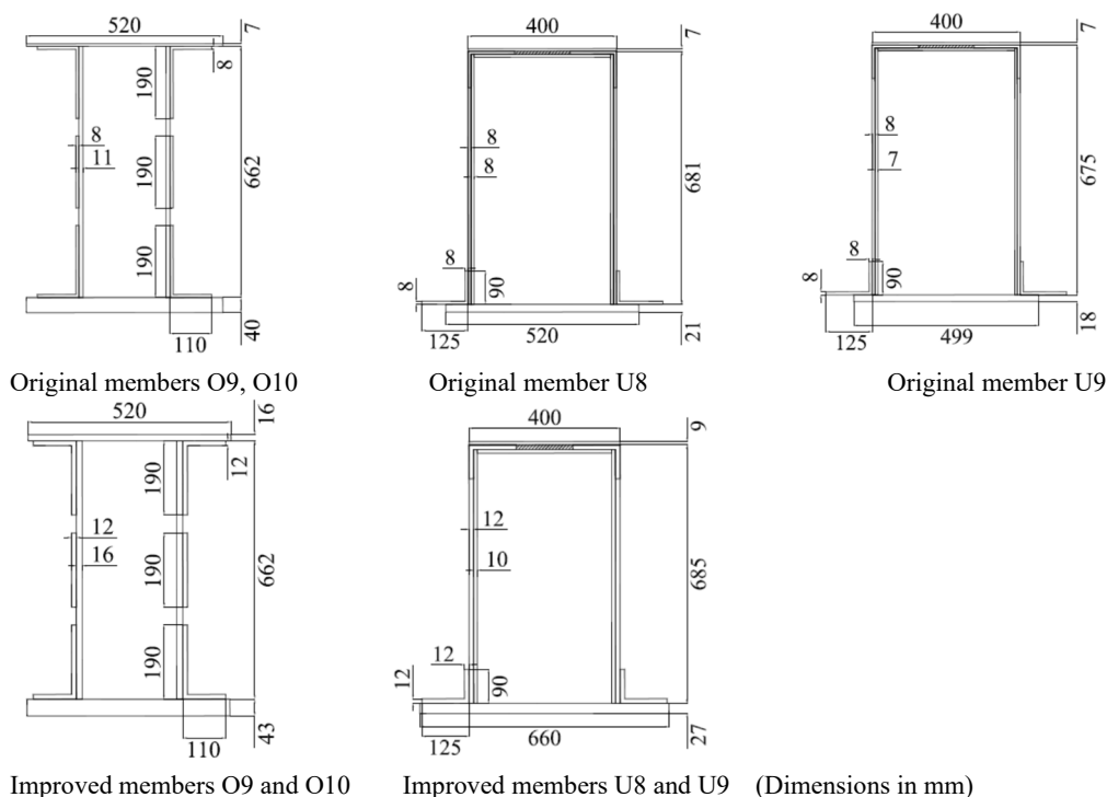
Fig.9 Estimated cross sections of original and improved members to resist dead load for damage structure (E1 damage).
