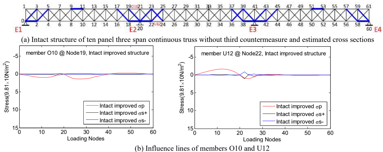
Fig.21 Influence lines of intact structure for members O10 and U12 in ten panel three span continuous truss bridge without third countermeasure and estimated cross sections.
