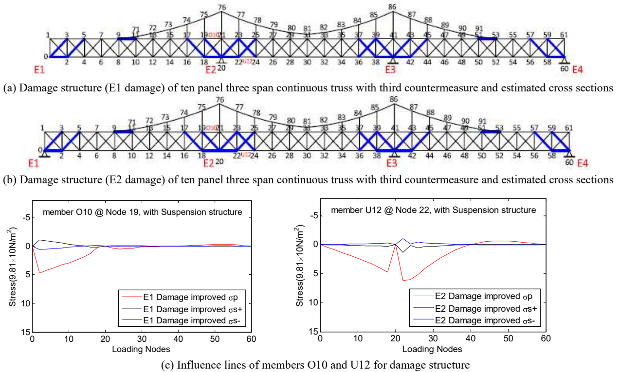
Fig.22 Influence lines of damage structure for members O10 (E1 damage) and U12 (E2 damage) in ten panel three span continuous truss bridge with third countermeasure and estimated cross sections.
