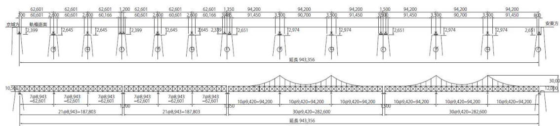
Fig.11 Longitudinal profile of Yalu river bridge 1) .
