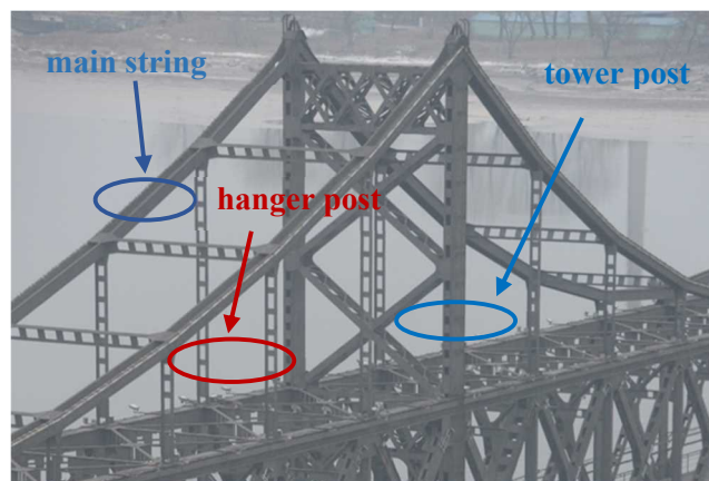
(a) Suspension structure of Yalu river bridge (Photo taken by Prof. Y. Takahashi)
