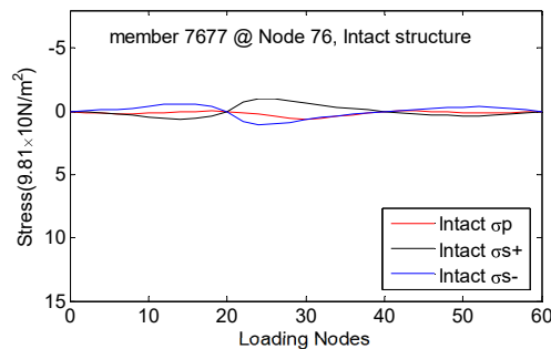
(a) Influence lines for curve member string
