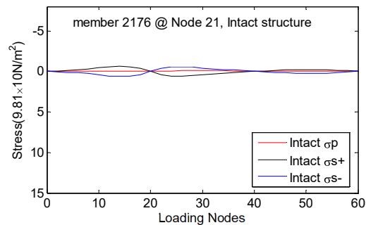
(b) Influence lines for tower post
