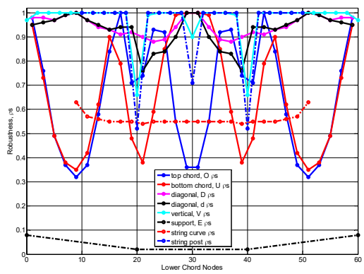
(c) Robustness for displacement
