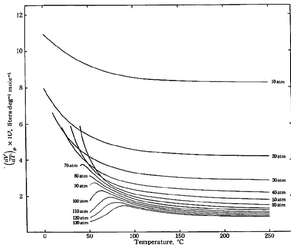
Fig. 3 The thermal expansion coefficient of acetylene at constant pressure
