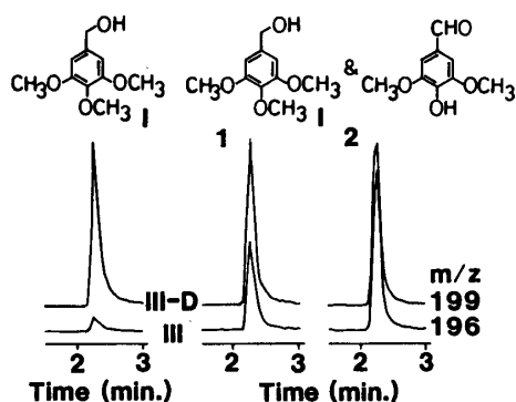
Fig. 1. Mass chromatograms of the M^+ regions of the degradation product III ( m/z 196) and internal standard III-D ( m/z 199). Internal standard ( 2 \mu\text{g} ) was added to the culture before extraction.
