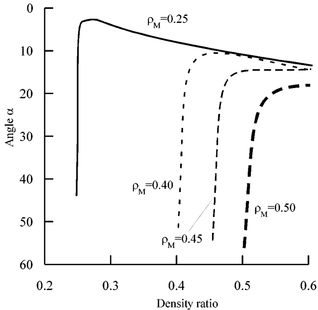
Fig. 8. Relationship between average angle \alpha and density ratio during transverse compaction.
