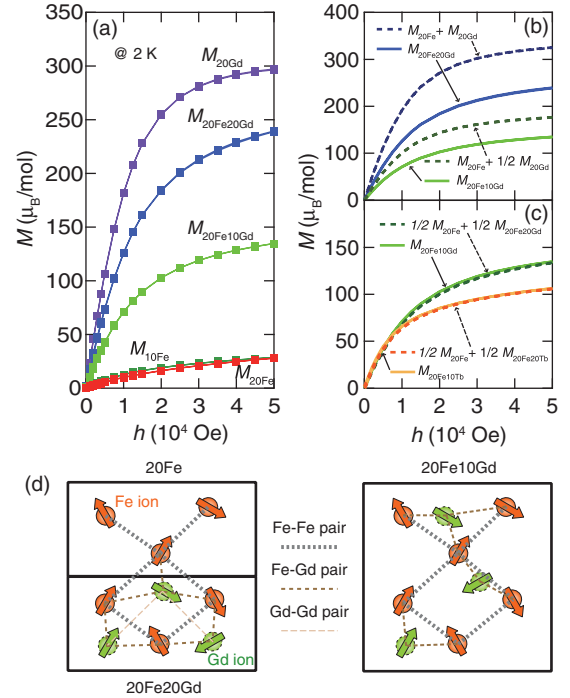
FIG. 5. (Color online) (a) The magnetic-field dependence of magnetization at 2 K for 20Gd, 20Fe20Gd, 20Fe10Gd, 20Fe, and 10Fe glasses, M_{20Gd} , M_{20Fe20Gd} , M_{20Fe10Gd} , M_{20Fe} , and M_{10Fe} , respectively. Plotted against magnetic field are (b) M_{20Fe20Gd} , M_{20Fe} + M_{20Gd} , M_{20Fe10Gd} , and M_{20Fe} + \frac{1}{2}M_{20Gd} and (c) M_{20Fe10Gd} , \frac{1}{2}M_{20Fe} + \frac{1}{2}M_{20Fe20Gd} , M_{20Fe10Tb} , and \frac{1}{2}M_{20Fe} + \frac{1}{2}M_{20Fe20Tb} . (d) Schematic models for M_{20Fe10Gd} and \frac{1}{2}M_{20Fe20Gd} + \frac{1}{2}M_{20Fe} are illustrated in the right and left panels, respectively.
