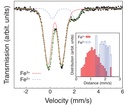
FIG. 1. (Color online) ^{57}\text{Fe} Mössbauer spectrum for 20Fe glass at room temperature. Experimental and computed absorption spectra are indicated by dots and the solid line, respectively. Calculated spectra attributed to \text{Fe}^{3+} and \text{Fe}^{2+} are represented by dashed lines. The inset shows distribution of distance between the peaks of doublets.
