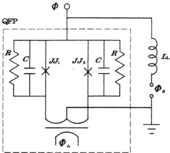
Fig. 1 QFP circuit
