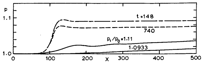
Fig. 11 Time-convergence of shock front for p_2/p_0=1.2 and n=1.0 ; --- unsteady shock at t=148 , -.- unsteady shock at t=740 , — stationary shock.
