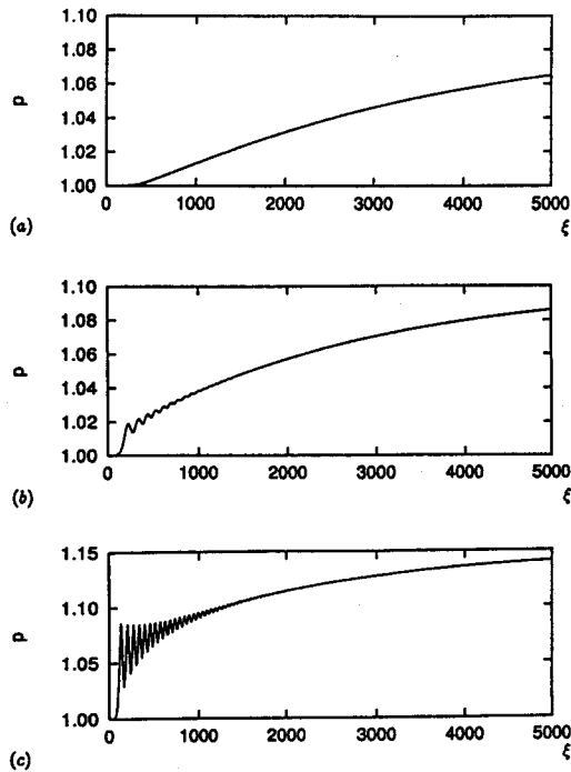
Fig. 5 Pressure distributions for \Psi=1.0+\psi_R ( \psi_r=0 ); a p_1/p_0=1.085 , b p_1/p_0=1.11 , c p_1/p_0=1.15 .
