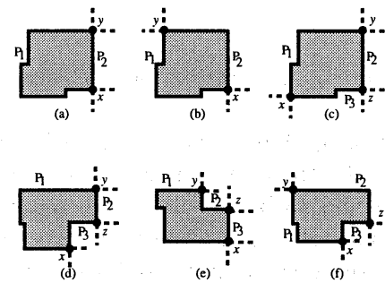
Figure 4: Illustration for feasible drawings.
