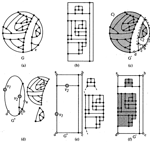
Figure 1: A plane graph and its orthogonal drawing.
