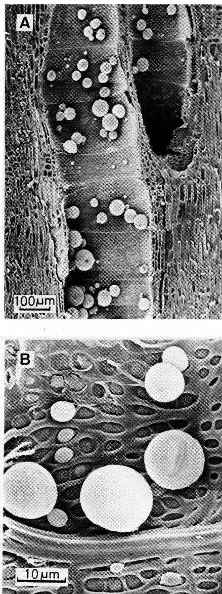
Fig. 2. Scanning electron micrographs of the inner surface of pore zone vessel collected at the beginning of October. (A) Tylosis buds are ballooned from pits all over the vessel inner surface, but (B) the occurrence is more abundant at the large and circular pits.
