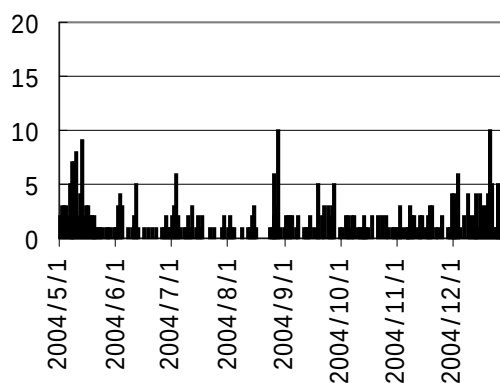
Fig. 4 Daily numbers of volcanic earthquakes at Kuchinoerabujima volcano counted by researcher
