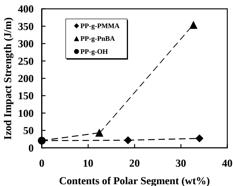
Figure 4. Plot of Izod impact strength versus content of polar segment.
