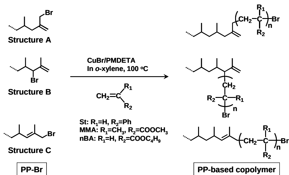
Scheme 2. Radical polymerization with PP-Br macroinitiator.
