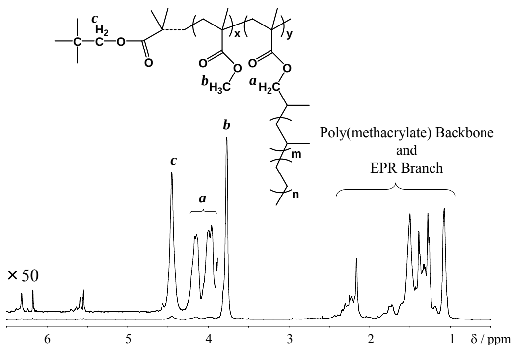
Figure 6. ^1\text{H} NMR Spectrum of PMMA- g -EPR star copolymer ( S1 ) (400 MHz in 1,2-Dichlorobenzene- d_4 at 120 ^\circ\text{C} ).
