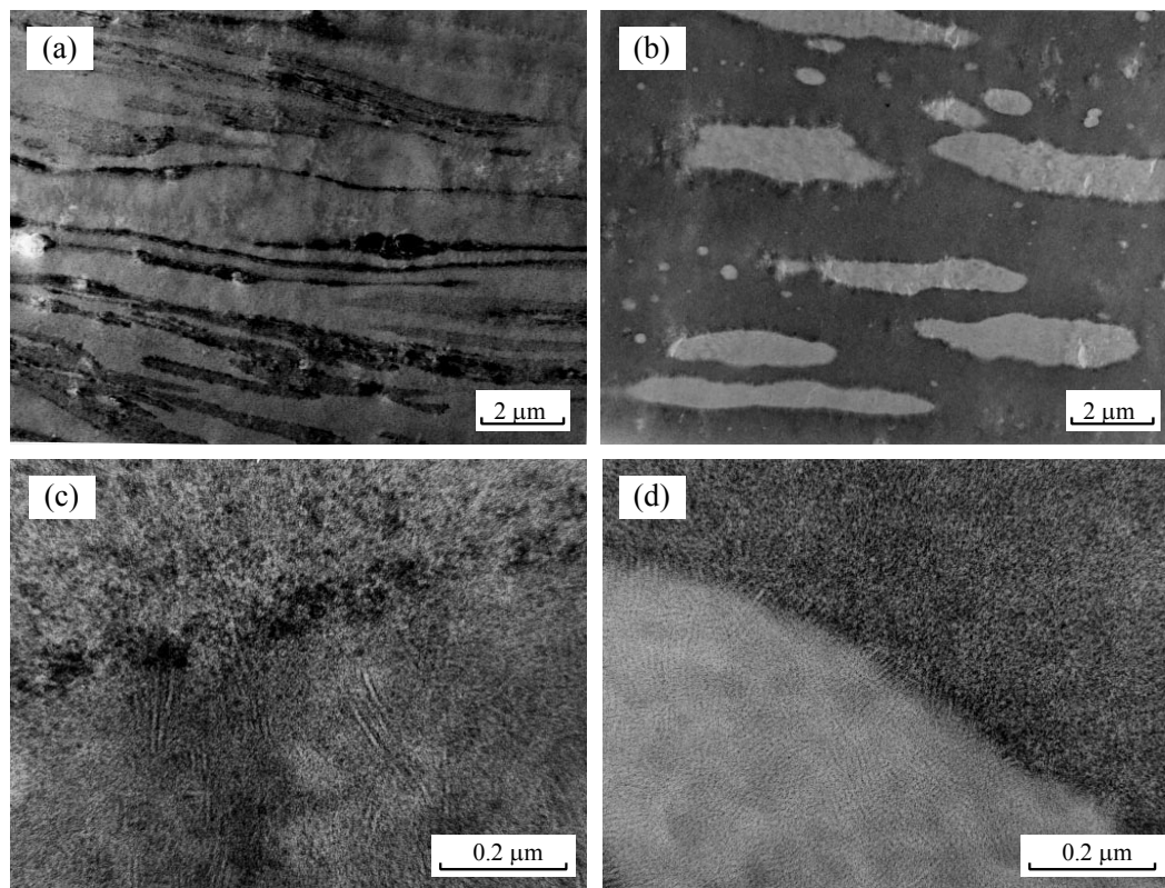
Figure 1. TEM micrographs at 10,000 magnification from (a) EPR- g -PP-2 produced by coupling reaction between PP-OH-2 and EPR- g -MAH-2 and (b) polymer blend consisting of py-PP and EPR- g -MAH-2 and at 150,000 magnification of (c) the EPR- g -PP-2 and (d) the polymer blend. The molar ratio of iPP segment to EPR segment is 6 to 1 in any of the both samples.
