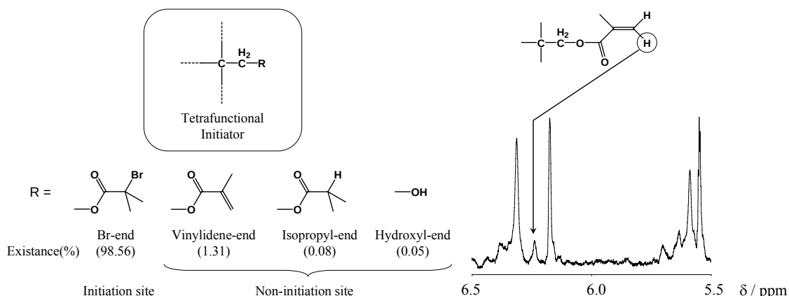
Figure 8. Magnified ^1\text{H} NMR spectrum of PMMA- g -EPR star copolymer ( S1 ) (400 MHz in 1,2-Dichlorobenzene- d_4 at 120 ^\circ\text{C} ).
