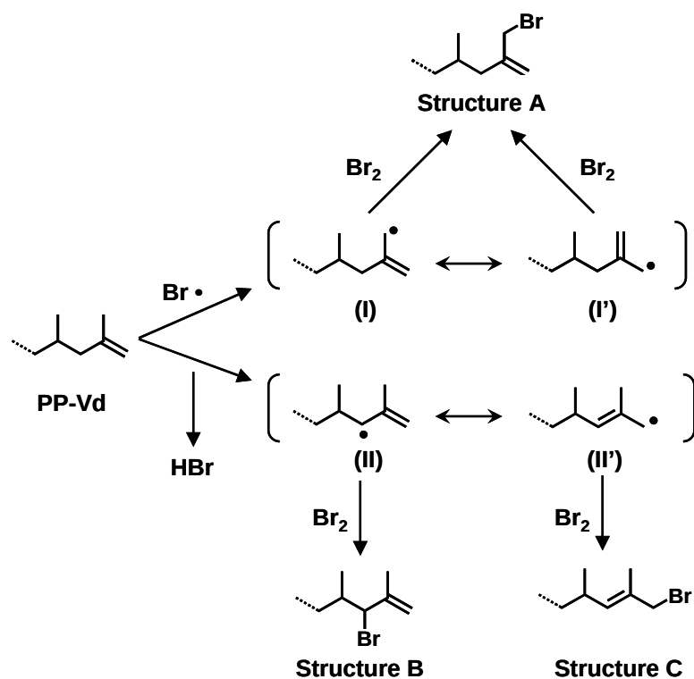
Scheme 1. Plausible structures of the allylic bromide moieties.
