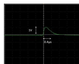
Fig.2 A pulse from B-10+ detector using a charge amplifier
