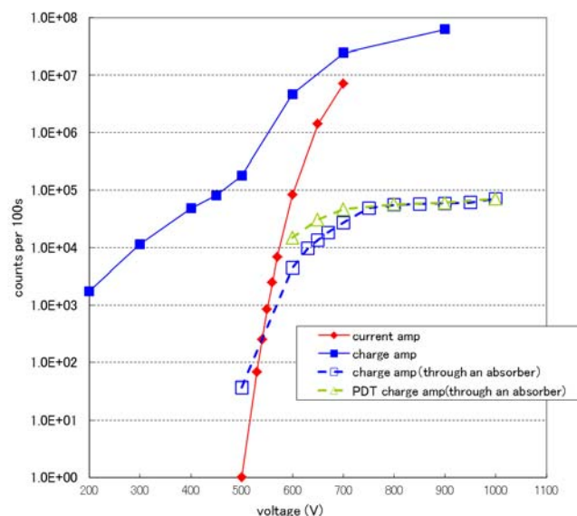
Fig.1 Plateau measurements of B-10+ detector with three kinds of amplifiers
