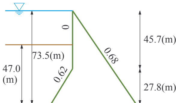
Fig.6 Designed basic section of A-dam with optimized parameters
