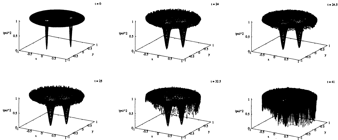
Figure 6: Evolution of the solution with \Delta t = 0.5 : Scheme 3 with (a, b) = (0.9, 0.5)
