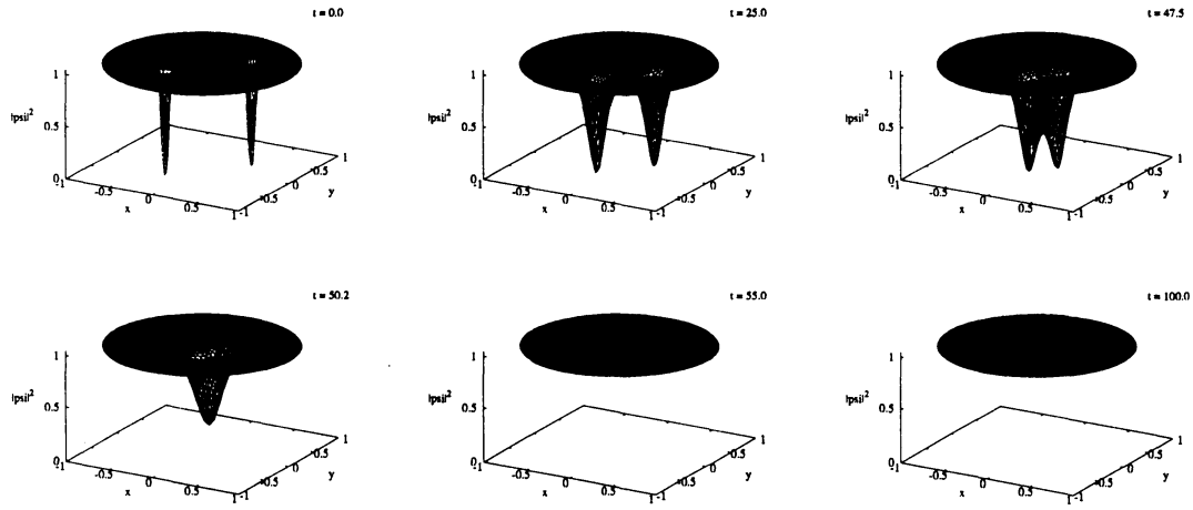
Figure 1: Evolution of the solution with \Delta t = 0.1 : the semi-implicit scheme and Scheme 3 with (a, b) = (2, -0.5)
