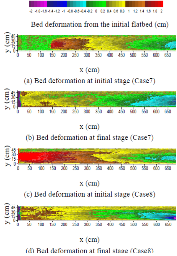
Fig.8 Bed deformation from the initial flatbed pre- and post- weir removal (Case7-8)
