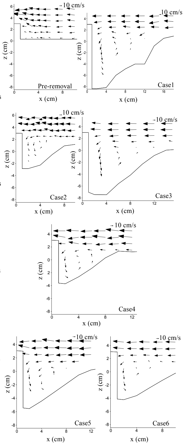
Fig.15 Velocity vectors ( u, w ) in the longitudinal cross-section B
