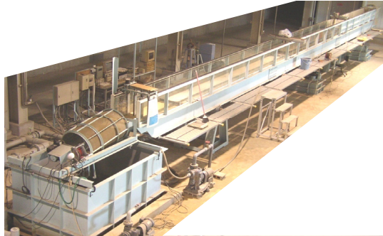
Photo 1 Experiment flume
