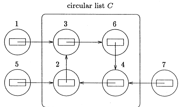
Figure 1: An example of graph G .
