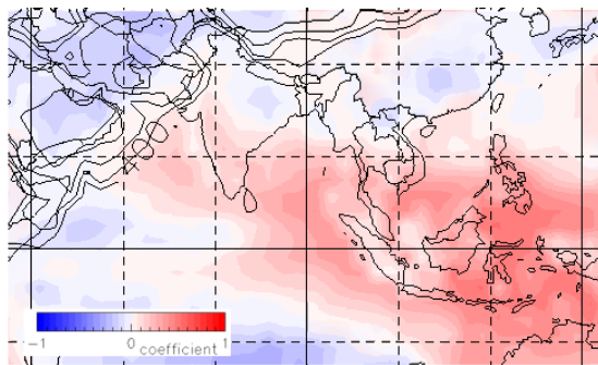
Fig.6 Spatial pattern of the regression coefficient of SOI in and around tropical Asia.
