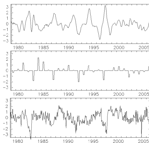
Fig.4 Time series of monthly objective values, DMI (top), MTG (middle), and SOI (bottom).
