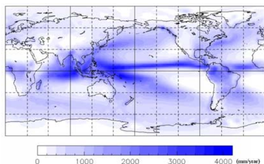
Fig.1 Spatial pattern of annual mean precipitation from 1979 to 2006, using GPCP datasets.
