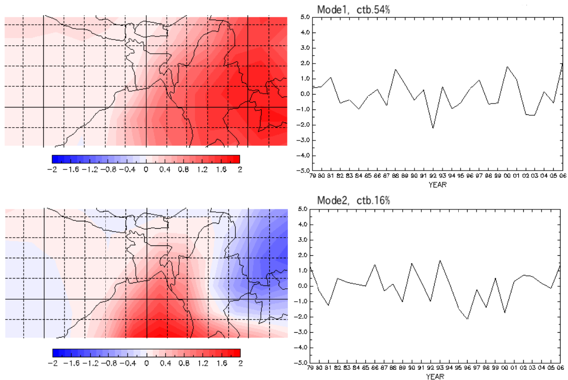
Fig.10 Spatial and temporal pattern of EOF analysis of annual mean precipitation anomalies.
