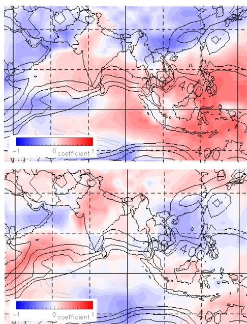
Fig.9 Spatial pattern of regression coefficient of SOI (top), DMI (bottom) only in DJF.
