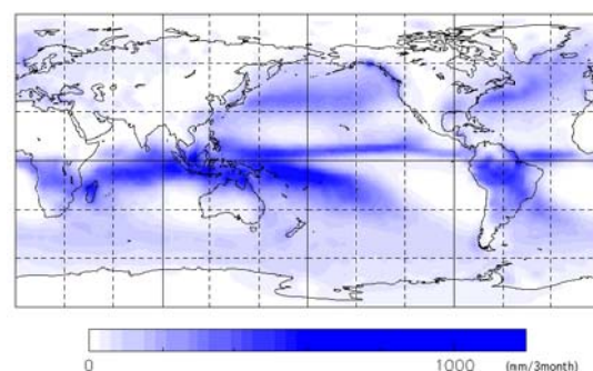
Fig.3 Spatial pattern of mean precipitation in DJF from 1979 to 2006.
