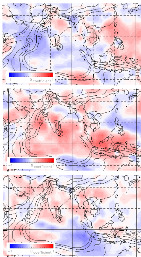
Fig.8 Spatial pattern of regression coefficient of MTG (top), SOI (middle), and DMI (bottom) only in JJA.
