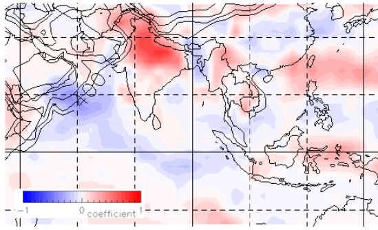
Fig.5 Spatial pattern of the regression coefficient of MTG in and around tropical Asia.
