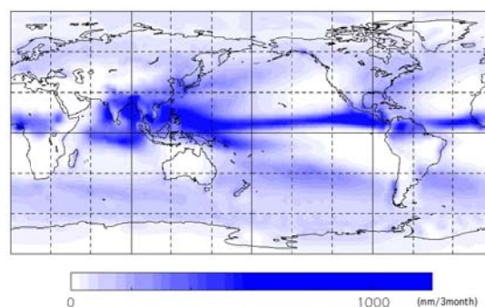
Fig.2 Spatial pattern of mean precipitation in JJA from 1979 to 2006.
