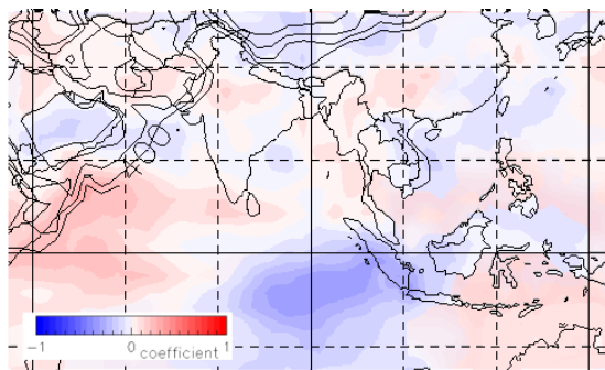
Fig.7 Spatial pattern of the regression coefficient of DMI in and around tropical Asia.
