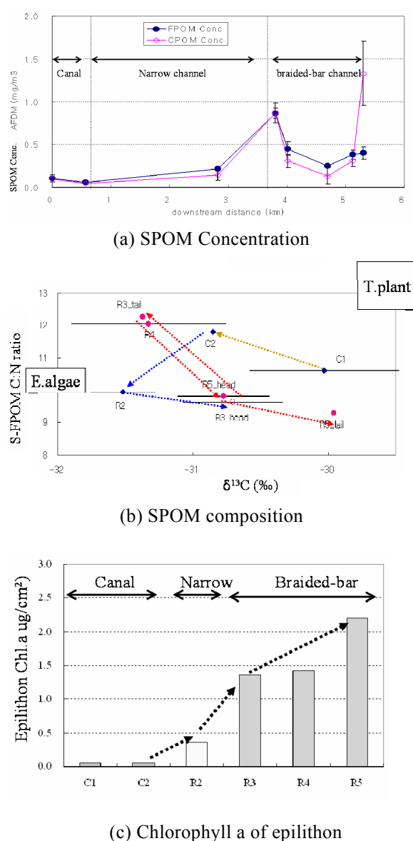
Fig.5 Downstream changes in SPOM concentration (a), trophic source composition (b) and algal production (c) passing through different channel forms in the Palar River.
