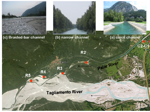
Fig.2 Study reaches in Palar River with longitudinal changes of channel forms. Canal from C1 to C2 (a), Narrow channel from C2-R2 to R3 (b), and Braided-bar channel from R3-R4 to R5 (c).
