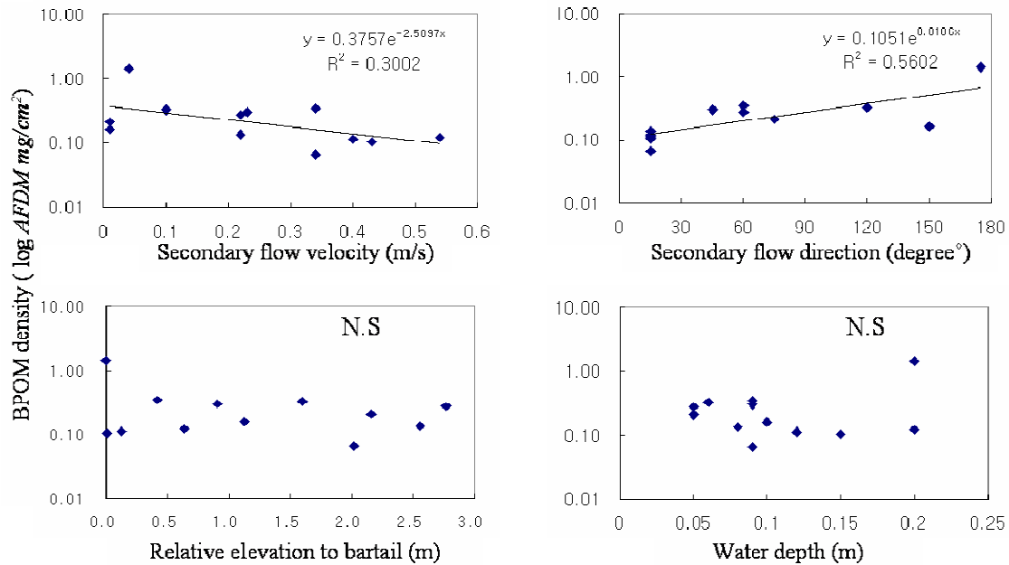
Fig 7. Relation of BPOM density to secondary flow velocity/direction, relative elevation and water depth of shallow area in an island bar unit.
