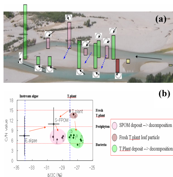
Fig.6 Spatial distribution of standing of fine BPOM stock and secondary flow velocity/direction (a), the arrow length and angle represent velocity and direction, respectively; Stable carbon isotope to C:N ratio value (b)
