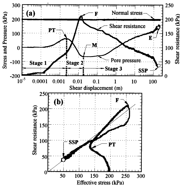
Fig. 4 Ring shear test on dense sand showing sliding surface liquefaction ( B_D=0.99 , D_r=95.2\% , \sigma = 196 kPa, PT: Phase Transformation; SSP: Steady State Point; F: Failure Point; E: Ending point). (a): Variation of pore pressure and shear resistance in relation to shear displacement; (b): Effective stress path.
