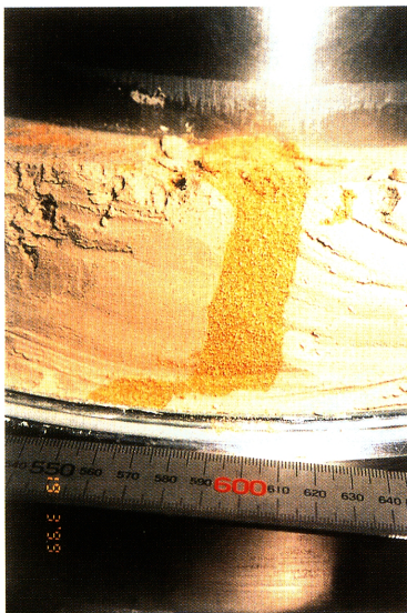
Fig. 10 Shear deformation of vertically inserted slice of Toyoura sand after 3-cm shear for the CT test shown in Fig. 9 ( B_D = 0.99 , D_r = 63.3\% ).
