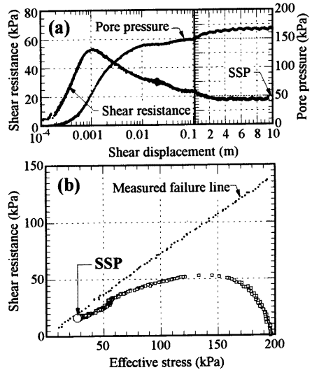
Fig. 3 Ring shear test on loose sand showing mass liquefaction phenomenon ( B_0=0.99 , D_r = 63.3\% ; SSP: Steady State Point). (a): Variation of pore pressure and shear resistance in relation to shear displacement; (b): Effective stress path.
