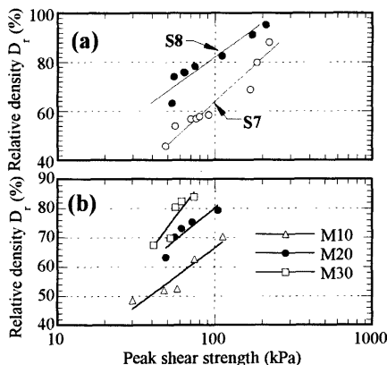
Fig. 17 Peak shear strength against D_r . (a): For the tests on S7 and S8; (b): For the tests on M10, M20, and M30.
