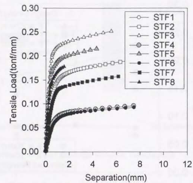
Fig. 4.13 Load-Separation Curves (Analysis)
