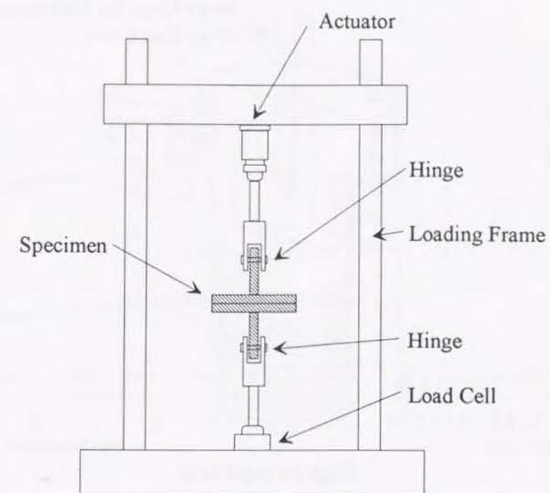
Fig. 4.3 Testing Setup
