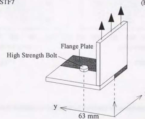
Fig. 4.17 Deformation of the Contact Surface
