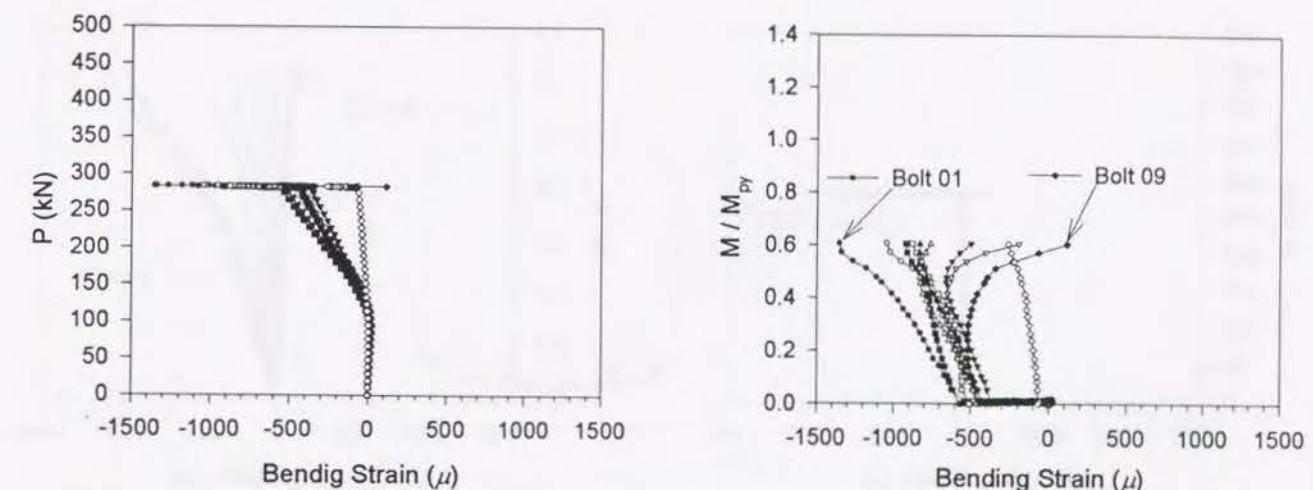
(i) Axial Tensile Load-Bending Strain Curves (ii) Bending Moment-Bending Strain Curves (b) CL-S-TH10-P10
