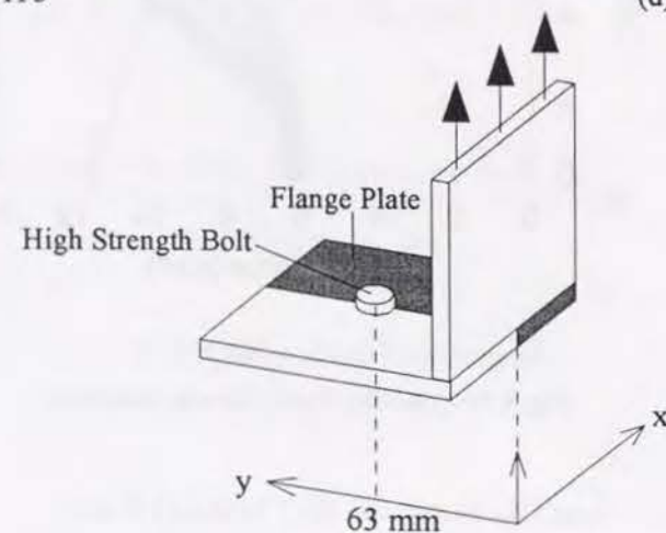
Fig. 4.17 Deformation of the Contact Surface (continued)
