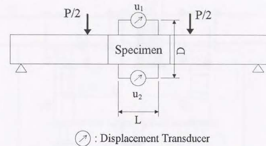
Fig. 6.4 Setup of the Displacement Transducer (BL Test)
