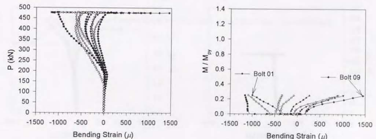
(i) Axial Tensile Load-Bending Strain Curves (ii) Bending Moment-Bending Strain Curves (c) CL-S-TH10-P17
