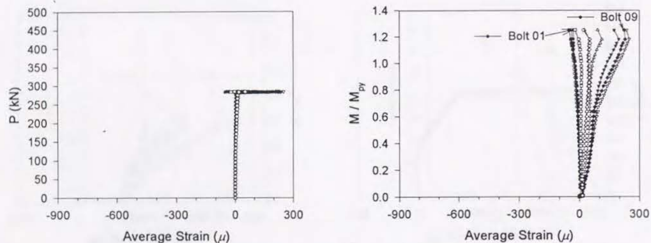
(i) Axial Tensile Load-Bolt Strain Curves (ii) Bending Moment-Bolt Strain Curves (e) CL-S-TH22-P10
