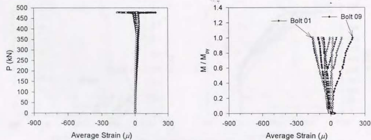
(i) Axial Tensile Load-Bolt Strain Curves (ii) Bending Moment-Bolt Strain Curves (f) CL-S-TH22-P17
