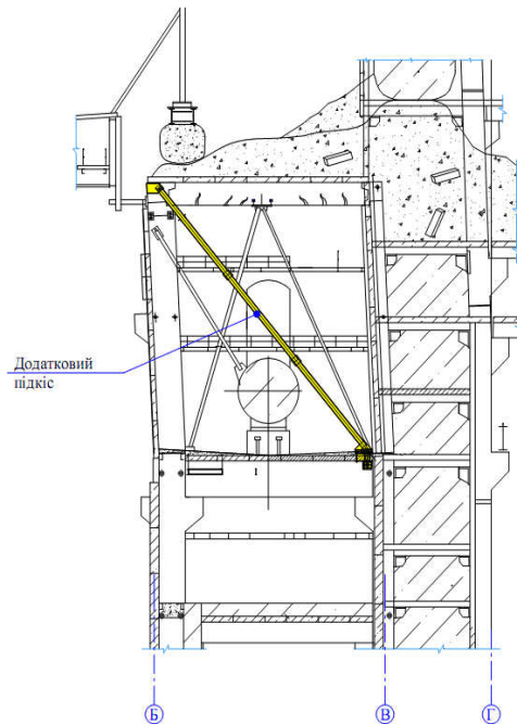
Fig. 6. Stabilization of the deaeration stack frame (measure #3)
