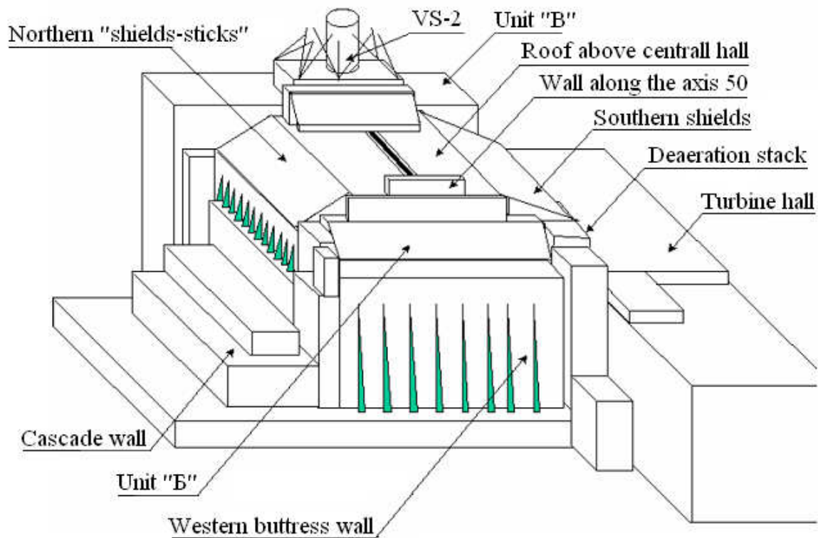
Fig. 4 “Shelter” Object protection structure location
