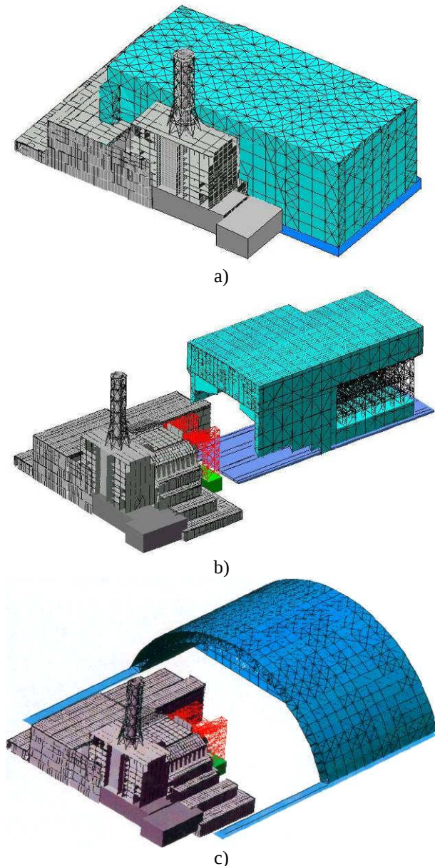
Fig 11. The main design systems for the new Safe Confinement (SC):
