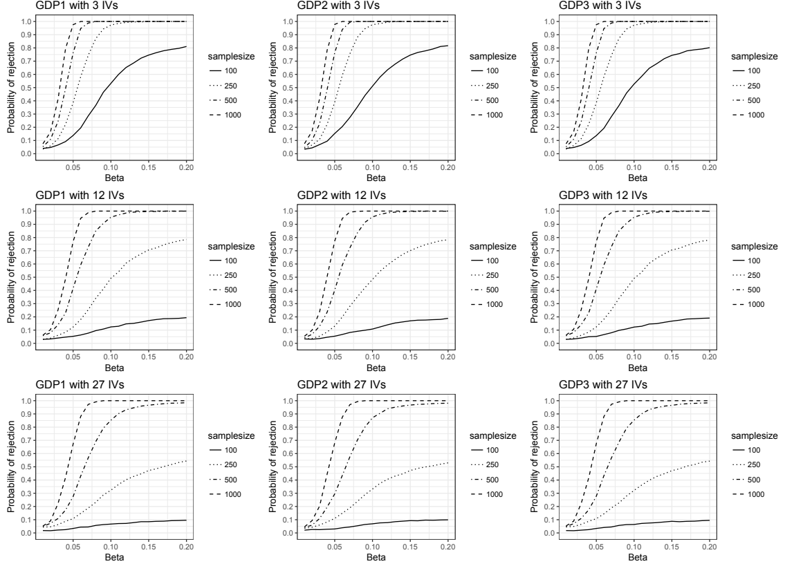
Figure 3: Power functions against non-smooth alternatives. Notes: Reported are fractions of rejection of the null hypothesis in 1000 simulation runs.
