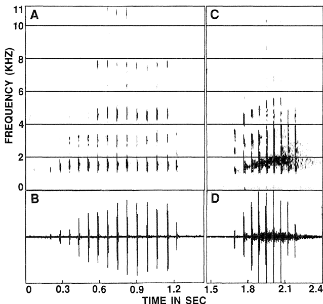
FIG. 2. Sonograms (A, C) and sound wave forms (B, D) of advertisement calls of Polypedates dugritei (A, B, recorded at 4.0°C; C, D recorded at 8.0°C).
