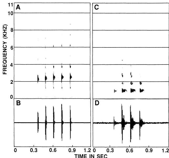
FIG. 1. Sonagrams (A, C) and sound wave forms (B, D) of advertisement calls of Polypedates chenfui (A, B, recorded at 13.0°C) and P. omeimontis (C, D, recorded at 11.0°C).
