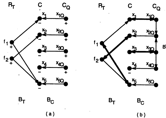
FIG. 1. Applying the CCF algorithm to the matrix of Example 1
