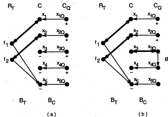
FIG. 2. Step A and Step B of the revised algorithm
