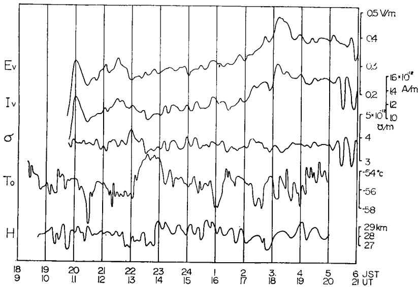
Fig. 6. Time variations of vertical electric field ( E ), current ( I ), conductivity ( \sigma ), air temperature ( T ) and balloon height ( H ). Electrical conductivity was calculated from Ohm's law ( \sigma=I/E ). Balloon height ( H ) was tracked by radar sounding.
