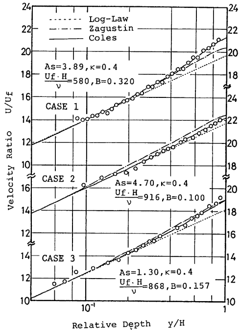
Fig. 1 Velocity distribution of clear water flow (smooth bed).
