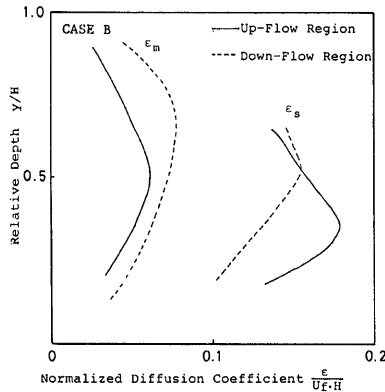
Fig. 13 Distribution of diffusion coefficient \varepsilon_m and \varepsilon_s .
