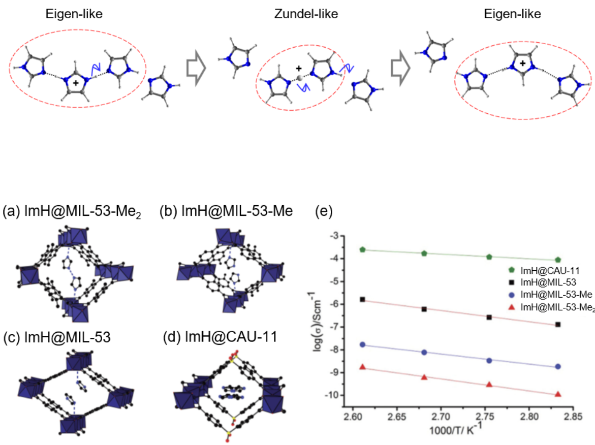
Figure 17. (a–d) crystal structures of ImH confined Al-based MOMs, ImH@MIL-53-Me 2 , ImH@MIL-53-Me, ImH@MIL-53, and ImH@CAU-11 (e) the Arrhenius plots of their proton conductivities. AlO 6 polyhedra are shown in dark blue, carbon atoms in black and nitrogen atoms in light blue. The potential hydrogen bonds are shown as dashed blue lines. Reproduced with permission. [104] Copyright 2016, Royal Society of Chemistry.
