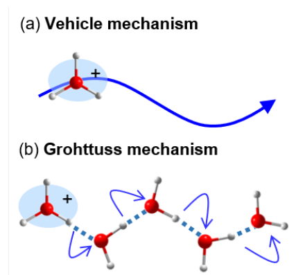
Figure 2. Schematic images of proton transport in the water medium. (a) Vehicle mechanism. (b) Grothuss mechanism.
