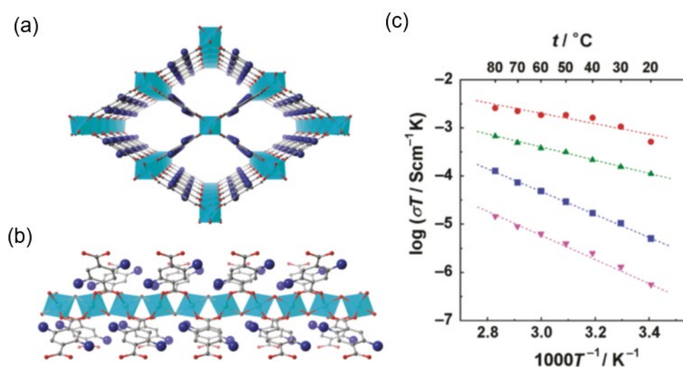
Figure 7. Crystal structures of MIL-53 deliveries. (a) Chains of corner-sharing MO_4(OH)_2 . (b) The structure along the channel axis. Al or Fe, C, O, and H are represented as light-blue, gray, red, and blue, respectively. The blue atoms show functional groups ( -NH_2 , -OH , or -COOH ). (c) Arrhenius plots of the proton conductivities of MIL-53(Al)-COOH (blue square), MIL-53(Al)-OH (pink triangle), MIL-53(Al) (green triangle), and MIL-53(Al)-NH 2 (red circle) under 95% RH conditions. Least-squares fits are shown as dotted lines. Reproduced with permission. [61] Copyright 2011, American Chemical Society.
