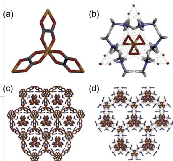
Figure 11. Crystal structures of \{[(\text{Me}_2\text{NH}_2)_3(\text{SO}_4)]_2[\text{Zn}_2(\text{ox})_3]\}_n (a) The tris-chelated D_3 -symmetric [\text{Zn}_2(\text{ox})_3]_2 subunit (b) 3D supramolecular [(\text{Me}_2\text{NH}_2)_3\text{SO}_4]^+_n net formed by hydrogen bonding between dimethyl ammonium cations and sulfate anions. (c) Packing structure of the MOM (d) Hydrogen bond interactions between dimethyl ammonium cations and sulfate anions in the MOM. Zn, C, N, O, S atoms are represented by orange, gray, blue, red, and yellow colors, respectively. Reproduced with permission. [70] Copyright 2013, John Wiley and Sons.
