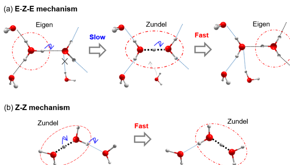
Figure 3. Schematic images of the elementary proton transport process in Grothuss mechanism. (a) E-Z-E type mechanism. (b) Z-Z type mechanism.
