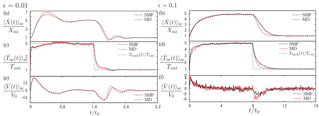
Fig. 4. The time evolutions of steady cycles for T_H/T_L = 5.0 . They are categorized into two types: damped oscillating type for \epsilon = 0.01 (left) and over-damped type for \epsilon = 0.1 (right). The time evolutions for the piston position [(a) and (b)], the temperature [(c) and (d)], and the piston velocity [(e) and (f)] are plotted. Time evolutions for the corresponding physical quantities for MD simulation (solid line) agree with those for the SMF model (dashed line).
