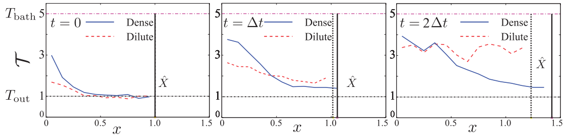
Fig. B1. The profiles of the temperature with the time interval \Delta t = 5.0 \times 10^{-3} \sqrt{MA/T_{\text{out}}} right after we change T_{\text{bath}} . The solid and dotted curves represent the profile of the temperature for dense ( d_{\text{in}}/\sqrt{A} = 0.1 ) and dilute ( d_{\text{in}}/\sqrt{A} = 0.01 ) gases, respectively. The vertical solid and dotted lines represent the position of the piston enclosing dense and dilute gases, respectively.
