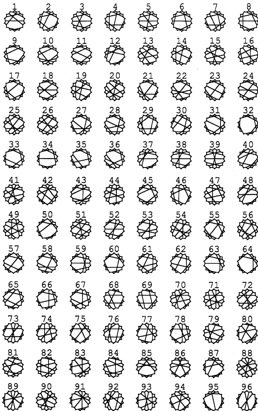
Figure 5: 14-gons with odd side-pairings
