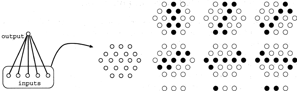
Figure 1: Neural network model.
