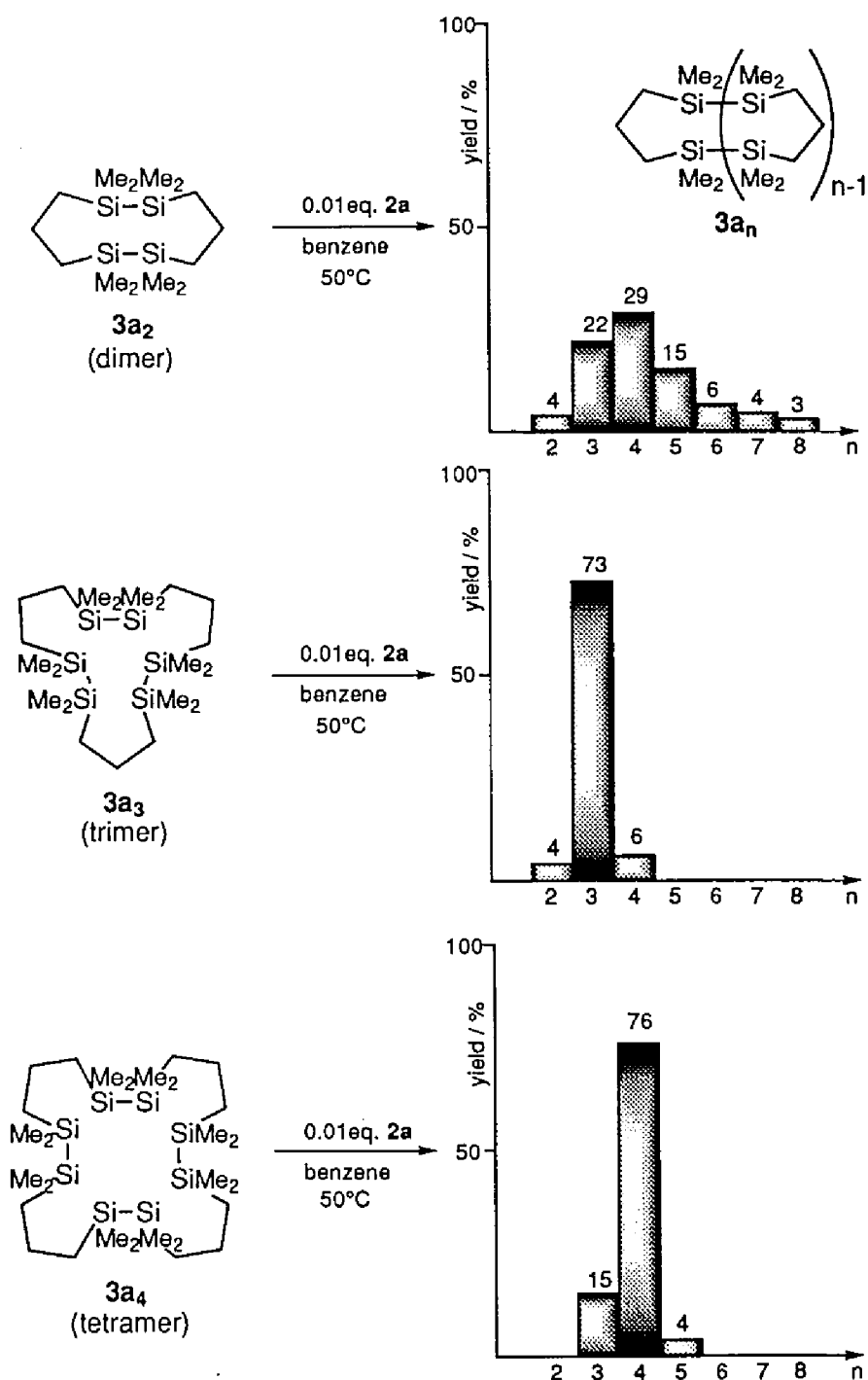
Scheme 2.
