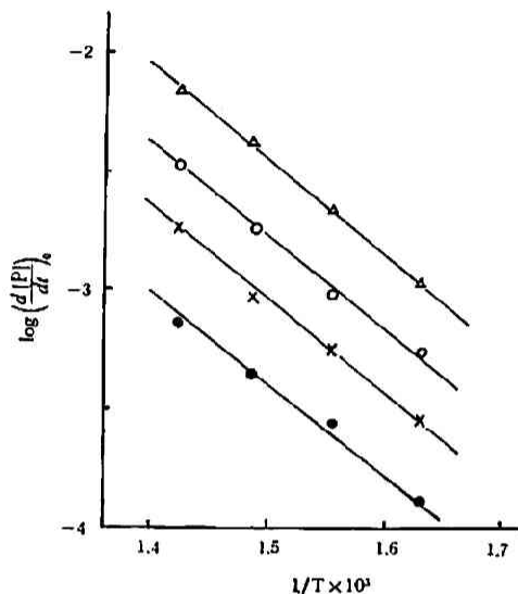
Fig. 4-2 Effect of temperature on the initial rate of phosgene formed at various CO/CH 3 Cl mole ratio 6 (Δ), 3 (○), 0.9 (×), 0.4 (●).
