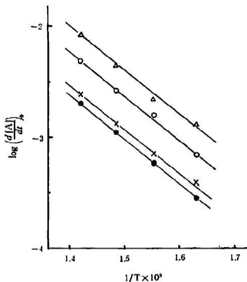
Fig. 4-1 Effect of temperature on the initial rate of acetyl chloride formed at various CO/CH 3 Cl mole ratio 6 (Δ), 3 (○), 0.9 (×), 0.4 (●).
