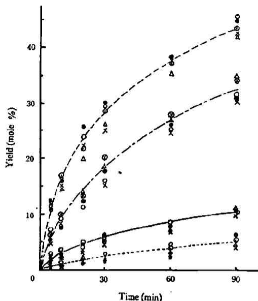
Fig. 3-5 Yield-time curves for hydrogen chloride at various temperature 430°C (---), 400°C (---), 370°C (—), 340°C (.....), and various CO/CH 3 Cl mole ratio 6 (⊙), 3 (Δ), 2 (○), 0.9 (×), 0.4 (●), 0 (⊗).
