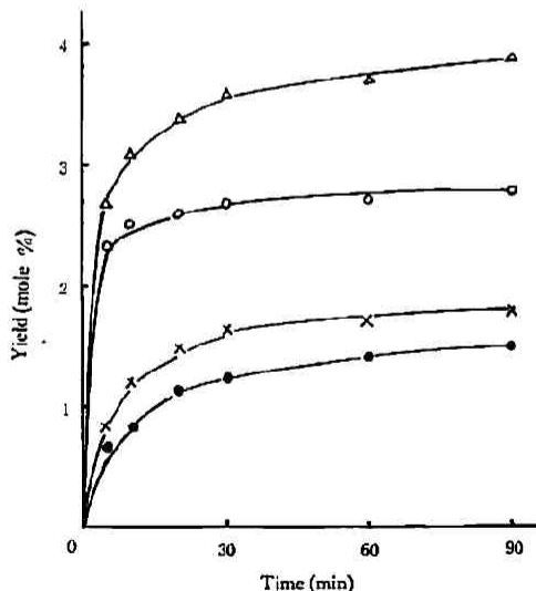
Fig. 3-2 Yield-time curves for acetyl chloride at constant \text{CO}/\text{CH}_3\text{Cl} mole ratio (6) and various temperature 430^\circ\text{C} ( \Delta ), 400^\circ\text{C} ( \circ ), 370^\circ\text{C} ( \times ), 340^\circ\text{C} ( \bullet ).
