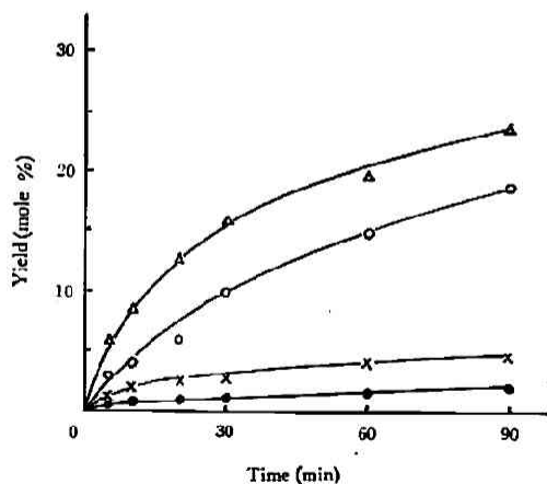
Fig. 3-7 Yield-time curves for methane at constant CO/CH 3 Cl mole ratio (0.4) and various temperature 430°C (Δ), 400°C (⊙), 370°C (×), 340°C (●).
