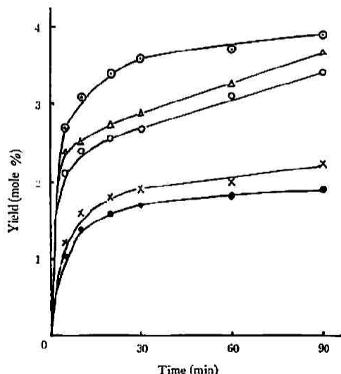
Fig. 3-1 Yield-time curves for acetyl chloride at constant temperature ( 430^\circ\text{C} ) and various \text{CO}/\text{CH}_3\text{Cl} mole ratio: 6 ( \odot ), 3 ( \Delta ), 2 ( \circ ), 0.9 ( \times ), 0.4 ( \bullet ).
