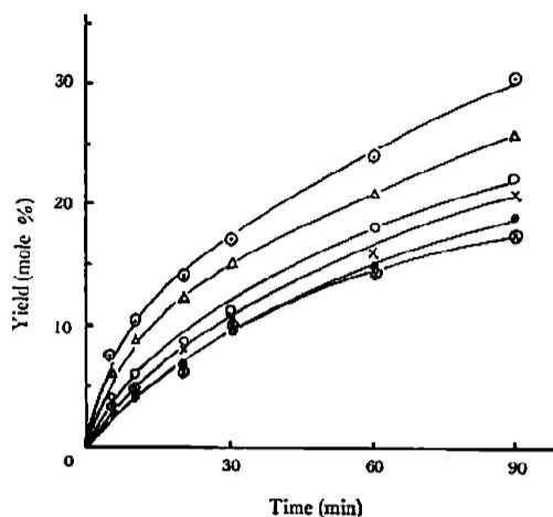
Fig. 3-6 Yield-time curves for methane at constant temperature (400°C) and various CO/CH 3 Cl mole ratio 12.8 (⊙), 6 (Δ), 2.5 (○), 1 (×), 0.5 (●), 0 (⊗).
