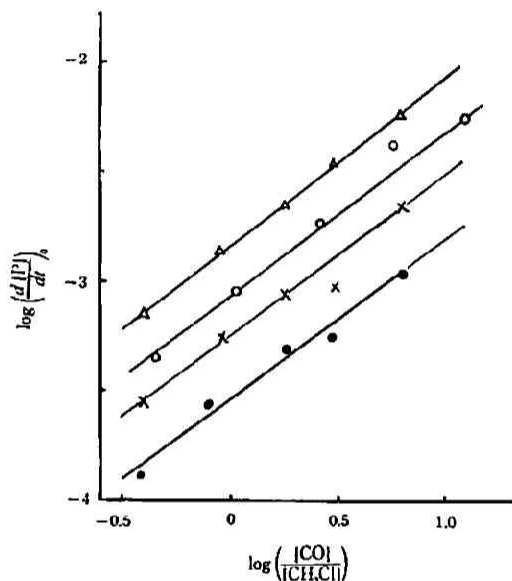
Fig. 5-2 Effect of \text{CO}/\text{CH}_3\text{Cl} mole ratio on the initial rate of phosgene formed at various temperature 430°C ( \Delta ), 400°C ( \circ ), 370°C ( \times ), 340°C ( \bullet ).
