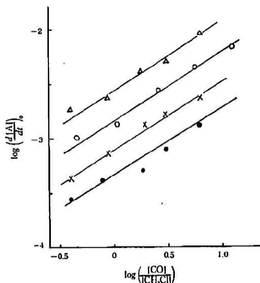
Fig. 5-1 Effect of \text{CO}/\text{CH}_3\text{Cl} mole ratio on the initial rate of acetyl chloride formed at various temperature 430°C ( \Delta ), 400°C ( \circ ), 370°C ( \times ), 340°C ( \bullet ).
