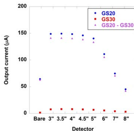
Fig. 2. Measurement results of the scintillator-based BSS.
