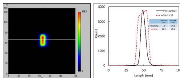
Fig.1. Real-time spatial distribution of the thermal neutron beam, and its beam profiles at E-3.
