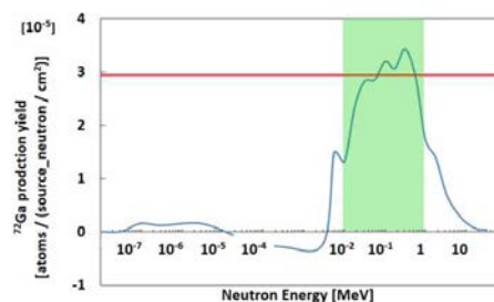
Fig. 2 Sensitivity of the second monitor.
