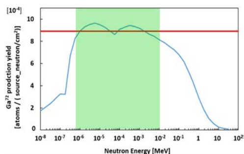
Fig. 1 Sensitivity of the first monitor.
