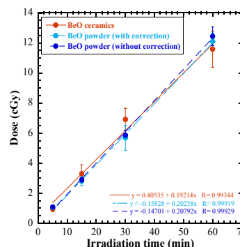
Fig.3 Gamma ray dose for irradiation time of BeO ceramic TLD and Na-doped BeO powder TLD.
