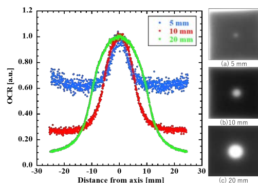
Fig.2 OCR of \text{Al}_2\text{O}_3 : Cr using Cd converter at mixed neutron irradiation mode in KUR-HWNIF.
