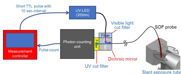
(a) Schematic illustration of deterioration monitor
