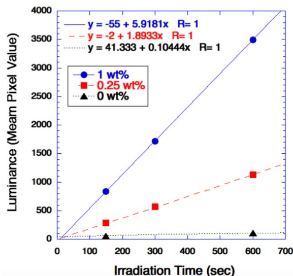
Fig. 2 Luminance value of boron-added liquid scintillator as a function of neutron irradiation time.
