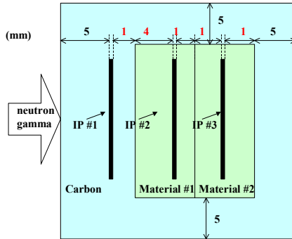
Fig. 1 Converter configuration.
