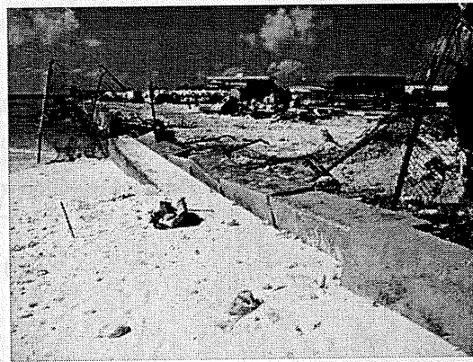
Photo 5.7 Damaged parapet of seawall
