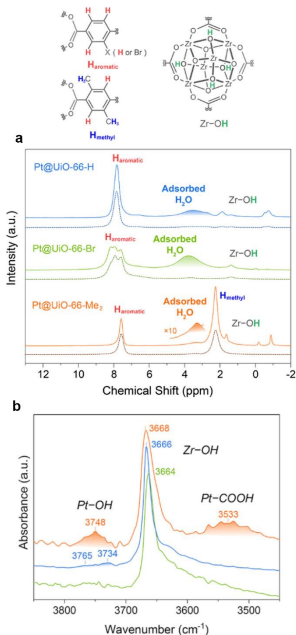
Fig. 9 (a) 1 H ultrafast (70 kHz) MAS NMR spectra (top, solid lines) and the corresponding 1 H- 1 H double-quantum NMR (DQNMN) spectra (bottom, dashed lines) of Pt@UiO-66-H (blue), Pt@UiO-66-Br (green), and Pt@UiO-66-Me 2 (orange) at room temperature. The peaks attributed to adsorbed H 2 O are highlighted. (b) In situ IR spectra on the condition of the WGS reaction for Pt@UiO-66-H (blue), Pt@UiO-66-Br (green), and Pt@UiO-66-Me 2 (orange). The gas flow rate was H 2 O/CO/N 2 = 4.5/0.4/15.1 sccm, and the temperature was 300°C. Reprinted with permission from Ref 57. Copyright 2020 American Chemical Society.
