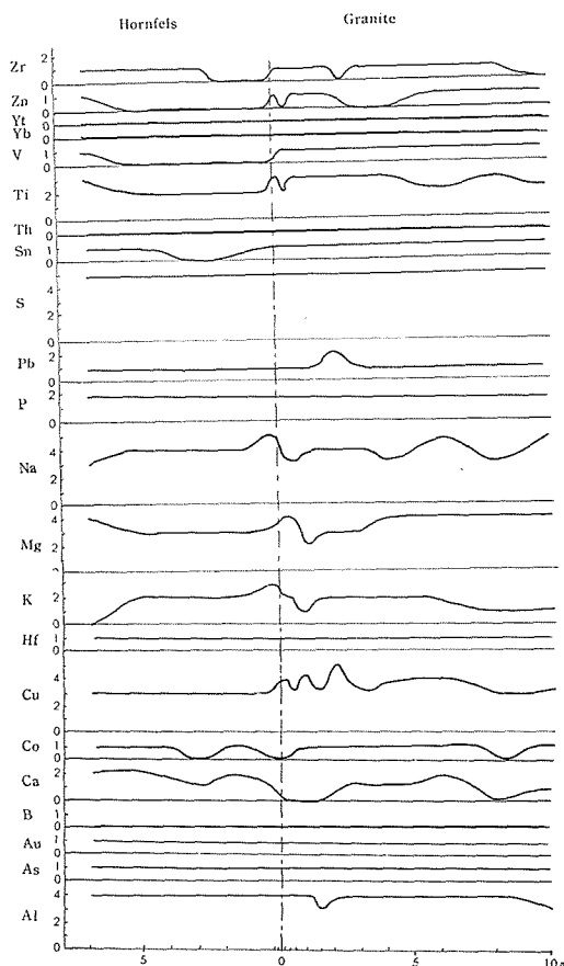
Fig. 3. Chemical element distributions with samples from Takamizu, Yamaguchi Pref. The ordinate being intensity of elements.
