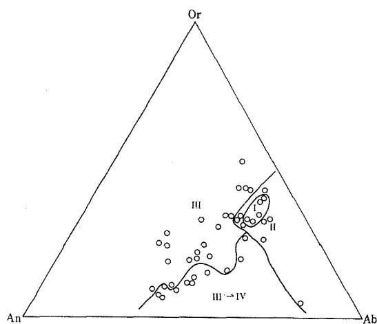
Fig. 9. Ternary diagram of the system, orthoclase-albite-anorthite relations obtained from norm calculation showing significant bearings on radioactivity types.
