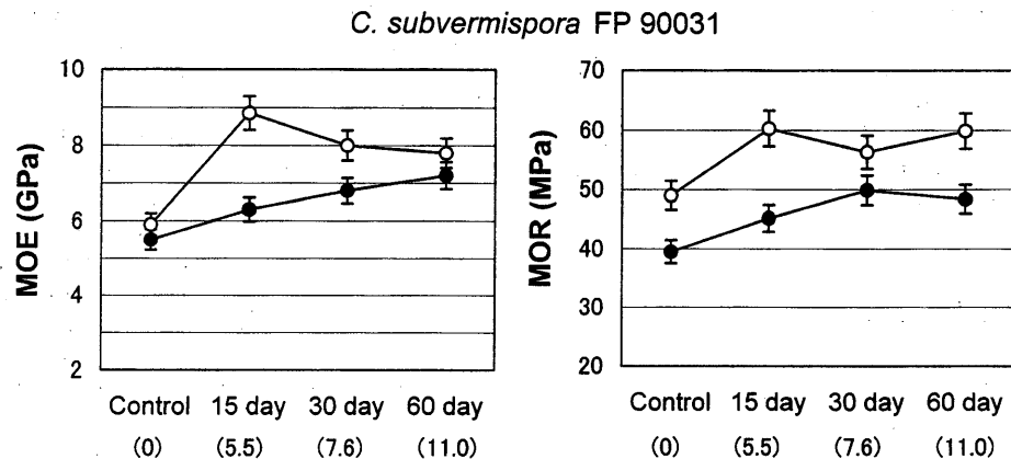
Fig. 2. Mechanical properties of moulding products made from radiata pine wood flour treated with C. subvermispora FP 90031 for 15, 30 and 60 days. Values in parentheses refer to percent total weight loss. Results are average value of 4 test samples with 95% confidence interval. —●— 130°C, —○— 160°C, 30 MPa, 10 min.
