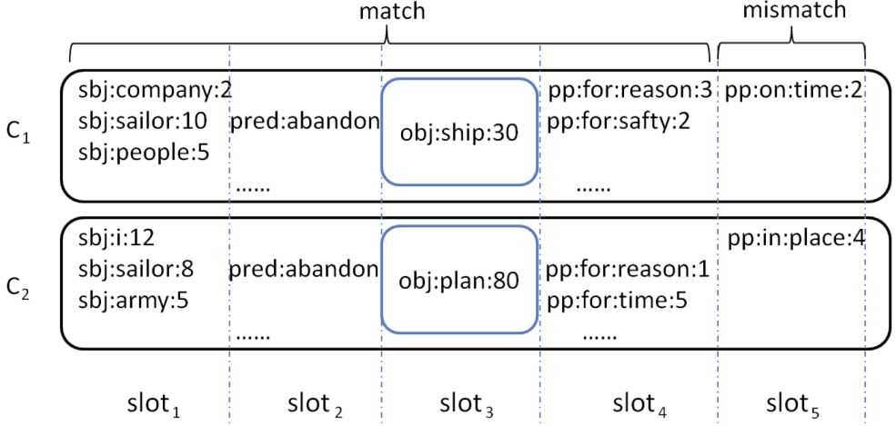
Figure 3.2: Initial cluster
