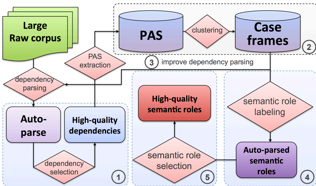
Figure 1.2: Framework overview
