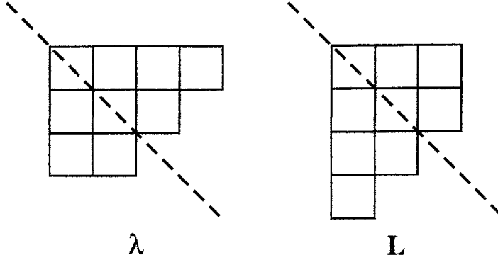
Figure 3: A pair of conjugate YD's.
