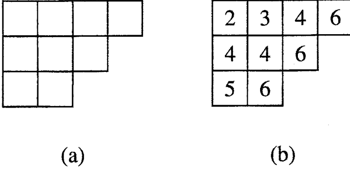
Figure 2: (a) Young diagram and (b) Young tableau T corresponding to the vicious walk in Figure 1.
