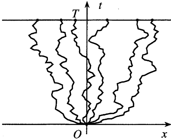
Figure 4: The process \mathbf{X}(t) , t \in [0, T] , starting from 0.
