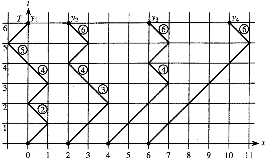
Figure 1: An example of vicious walk in the case N = 4, T = 6 .
