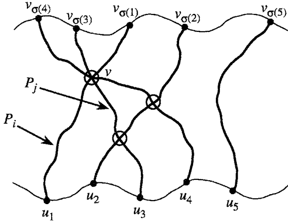
Figure 5: A configuration (\sigma, P_1, \dots, P_N) . The last intersecting vertex is denoted by v and lattice paths P_i and P_j are chosen, both of which pass through v .
