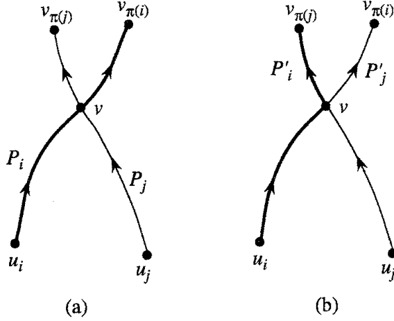
Figure 6: (a) Paths P_i and P_j . (b) Paths P'_i and P'_j .
