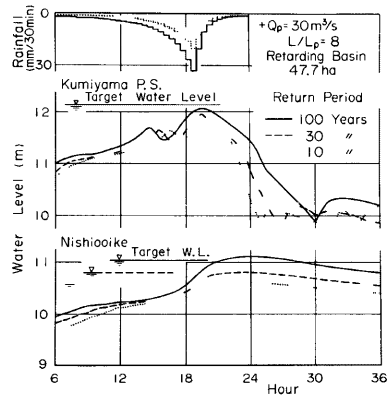
Fig. 15. Hydrographs of flood water level at Kumiya and Nishioike under some hypothetical counter-measures for flood in the future.
