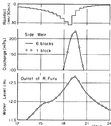
Fig. 7. Effects of the reach division in the reach of side weir of 150 m in flood routing on hydrographs of outflow and water level.
