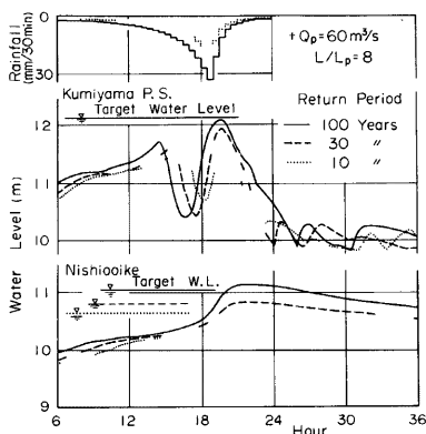
Fig. 13. Hydrographs of flood water level at Kumiyama and Nishiooike under some hypothetical counter-measures for flood in the future.
