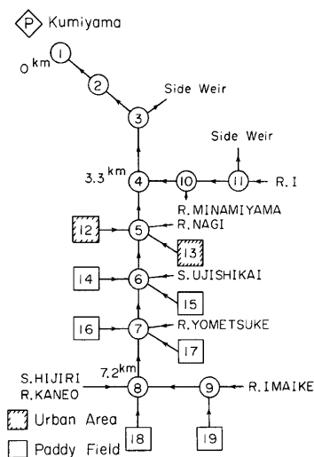
Fig. 5. Schematic diagram of inundation watershed of the Joudan zone in the future. In the examination of reach tank length, both side weirs are neglected.
