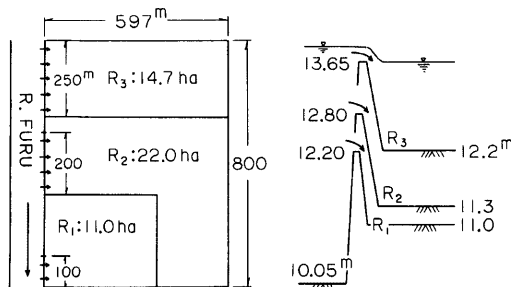
Fig. 14. Outline of the retarding basin and the highest water level for rainfall of 100 years return period.
