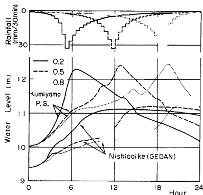
Fig. 10. Effects of the shape of hyetograph on flood hydrograph at a point. The value 0.2 in this figure, for example, means that the peak of hyetograph is situated at the time of 0.2 \times 24 \text{ hr} = 4.8 \text{ hr} from the beginning of rainfall.
