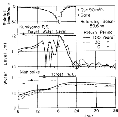
Fig. 16. Hydrographs of flood water level at Kumiya and Nishioike under some hypothetical counter-measures for flood in the future.
