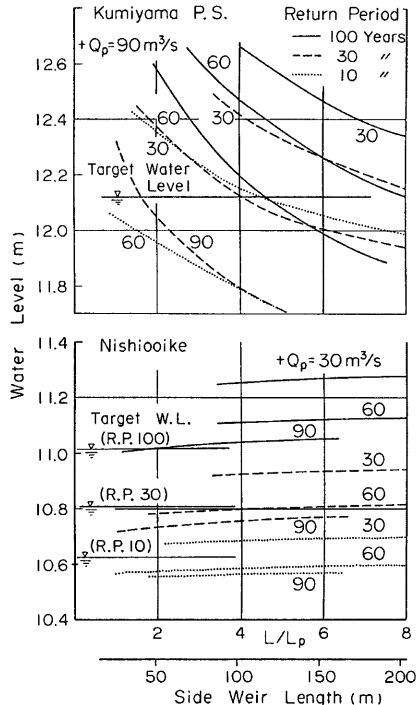
Fig. 12. The relations between the side weir length in the River Furu and the highest water levels at Kumiyama and Nishiooike under some hypothetical pump capacities, in which, +Q_p means added pump capacity.
