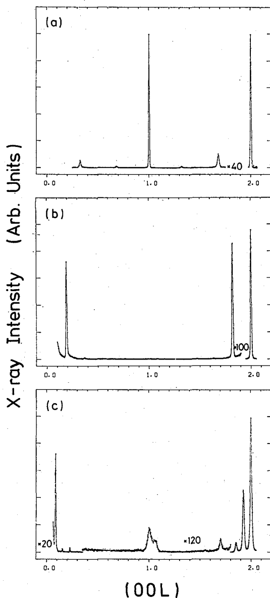
Fig. 1. X-ray diffraction patterns with the scattering vector normal to the film plane of (a) (\text{PbSe})_8(\text{SnSe})_8 , (b) (\text{PbSe})_8(\text{SnSe})_4 and (c) (\text{PbSe})_{13}(\text{SnSe})_{14} . These samples are typical ones for regions I, II and IV in the sample map shown in Fig. 3.
