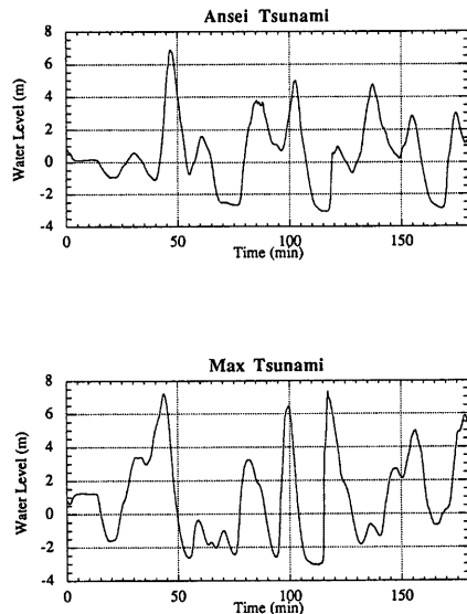
Fig. 16 Changes of water level with time
