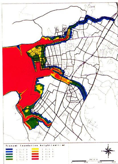
Fig. 20 Spatial distribution of maximum inundation depth due to the plausible maximum earthquake tsunamis (storm surge gate is closed)
