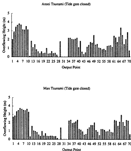
Fig. 15 Distribution of maximum differential water level over crown height of embankment (storm surge gate is closed)
